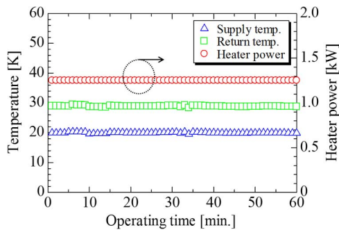
Fig. 6. Supply/return temperature of helium gas and the heat input from the dummy heater during the cooling capacity test at 20 K/30 K. Open triangles show the supply temperature, open squares the return temperature, and open circles the electric power of the dummy heater.
