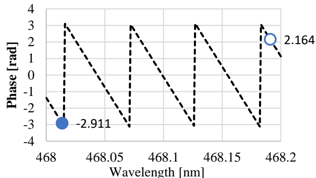
FIG. 6. A phase dependence of wavelength at case 2. A closed circle is phase -2.91 rad at Zn (468.014 nm) and an open circle is phase 2.164 rad at Ti (468.19 nm). A dashed line is extrapolation of \phi(\lambda) through 2 circles.
