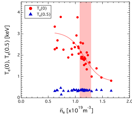
Figure 3. Density dependence on central( r/a = 0 ) and peripheral( r/a = 0.5 ) T_e .
