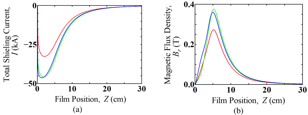
Figure 9: Dependences of (a) the total shielding current I and (b) r -component B_r(Z, R, t) of the magnetic flux density on the film position Z .
