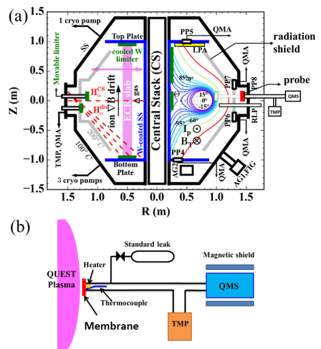
Fig. 1 (a) Schematic view of QUEST cross-section, and (b) schematic diagram of the permeation setup.
