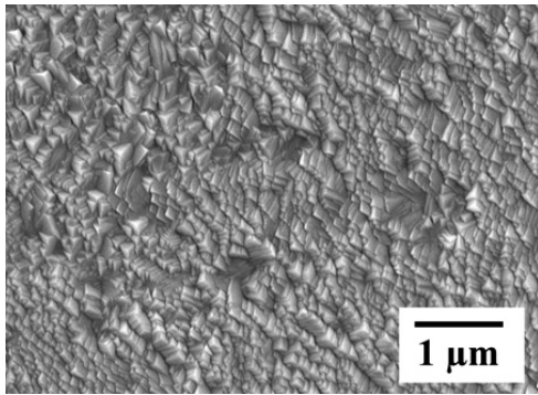
Fig. 2 SEM image of the SP-W coatings surface.
