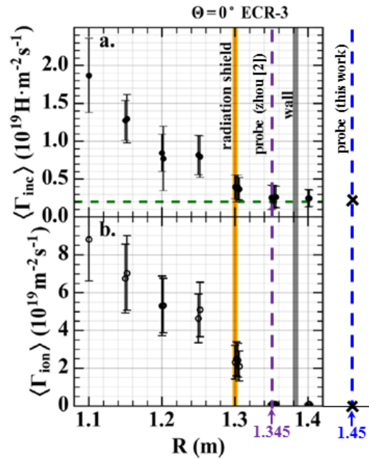
Fig. 3 Radial profiles of hydrogen incident flux ( \Gamma_{\text{inc}} ) by a reciprocate PdCu permeation probe (indicated as PP8 in Fig. 1) and ion flux ( \Gamma_{\text{ion}} ) by a reciprocate Langmuir probe (indicated as RLP in Fig. 1) in QUEST (reedit from Ref. [6]).
