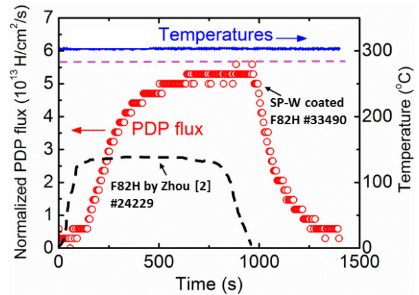
Fig. 4 Comparison of hydrogen PDP through the SP-W coated F82H and bare F82H membranes in a 910 s steady-state wall conditioning discharge. The thicknesses of SP-W coatings and F82H substrate are 0.5 \mu\text{m} and 0.25 mm, respectively.
