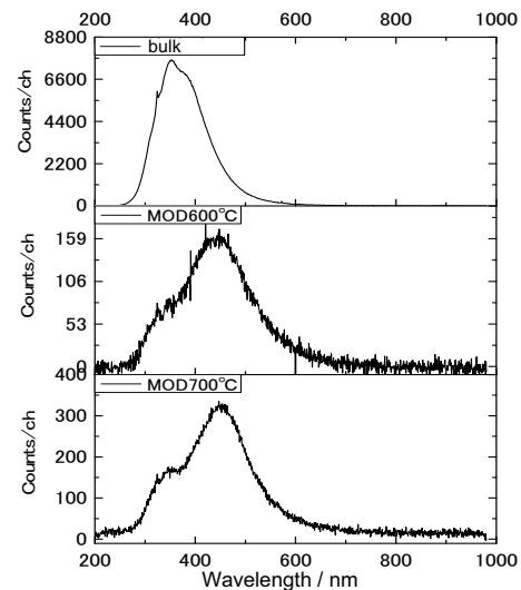
Fig. 1. SEM-CL spectra of sintered bulk \text{Y}_2\text{O}_3 sample and \text{Y}_2\text{O}_3 coating sample fabricated by MOD method.
