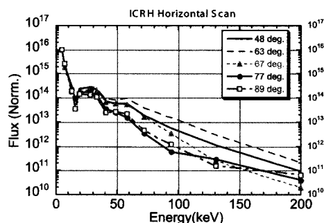
Fig. 5 (a) The energy spectrum of each scanning angle. The vertical error bars are smaller than symbols.
