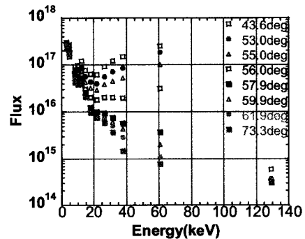
Fig. 3 (b) Energy spectrum of each pitch angle obtained by Fig. 3(a).
