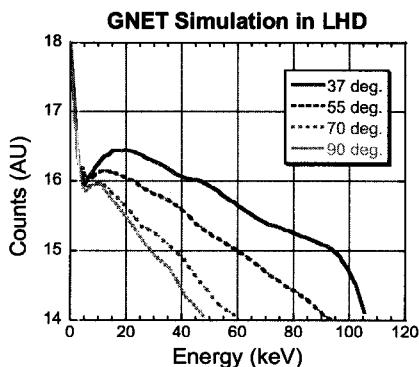
Fig. 4 GNET Simulation in NBI plasma.
