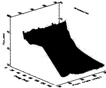
Fig. 3 (a) The spatial-resolved neutral particle energy spectrum in NBI long discharge.
