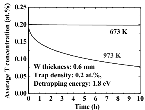
Fig. 2 Results of T release simulation with the TMAP4 program.
