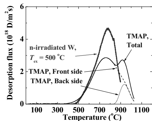
Fig. 1 TDS spectrum of D from neutron-irradiated W (0.025 dpa) 1-3 and the result of simulation with the TMAP4 program. The activation energy for detrapping, E_{det} , was set to 1.83 eV in the simulation.
