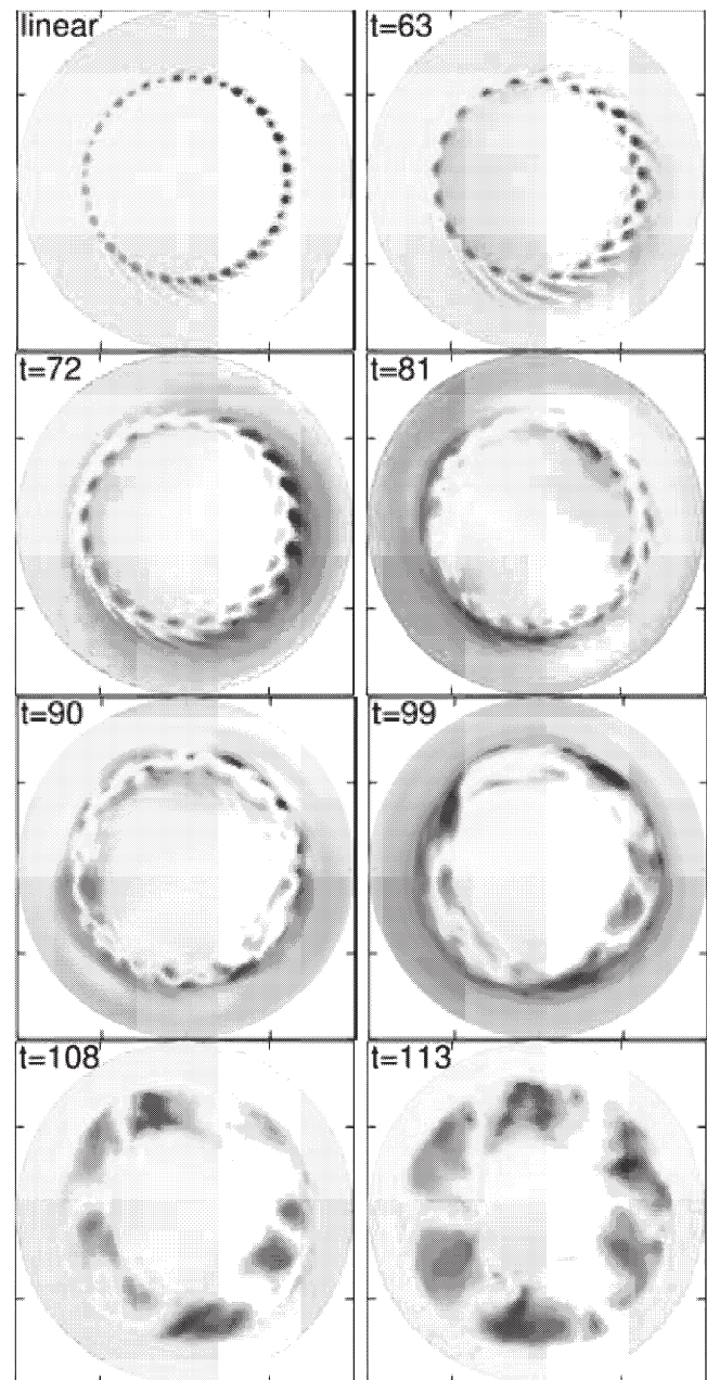
Fig.1. Time evolution of the electric potential on a poloidal section, where the time is normalized by the ion thermal transit time. The micro-instability dominates the linear evolution, then its ballooning structure is deformed by the zonal flow at t=72 and the instability is suppressed by the flow. Next, the m=3 tearing mode arises at t=99 , finally the turbulence due to micro-instability expands over the plasma at t=113 .
