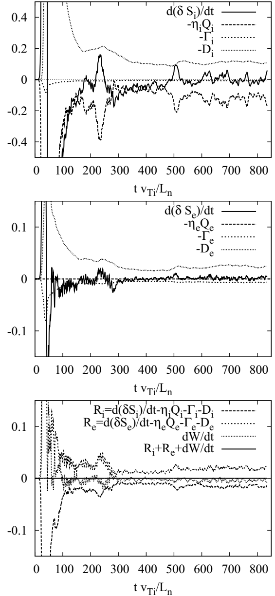
Fig. 1: Time evolution of each term in the entropy balance equation for the mass ratio m_i/m_e = 1836 .
