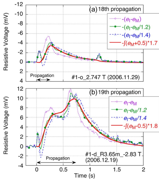
Fig. 7. The estimated normal components for the 18th (a) and 19th (b) propagation of a normal-zone.
