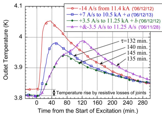
Fig. 3. Temperature rises at the outlet of helical coil by excitation, where a is “+1.4 A/s to equivalent 11.1 kA”, and b is “+0.7 A/s to equivalent 11.5 kA.”
