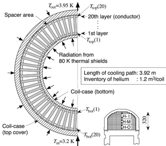
Fig. 8. The schematic drawing of a cooling path of the helical coil. One coil has ten paths.
