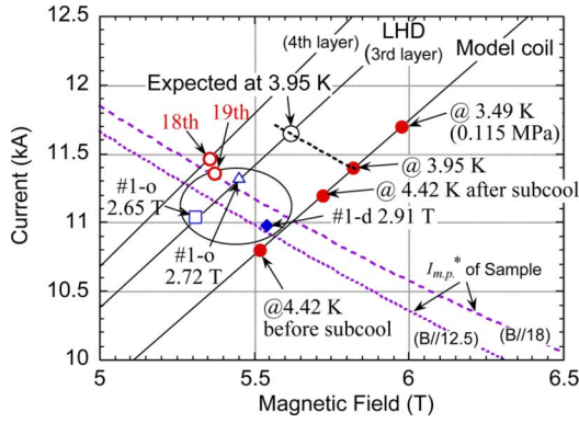
Fig. 4. Minimum current for a normal-zone propagating in the LHD helical coil and the model coil. The maximum field in the last turn of the third layer is used for the LHD helical coil.
