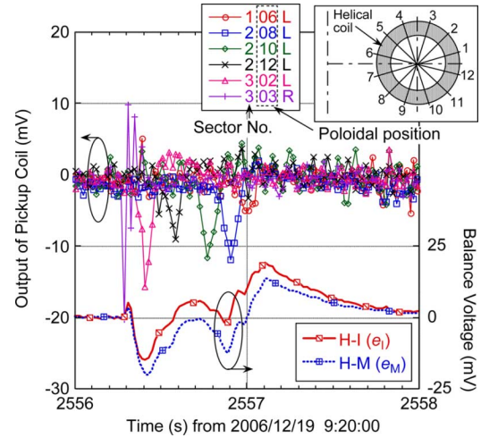
Fig. 6. Balance voltage of the helical coils and output of pickup coils during the 19th propagation of a normal-zone. The sector number means the toroidal position, and 1st and 6th are located at north and south, respectively.
