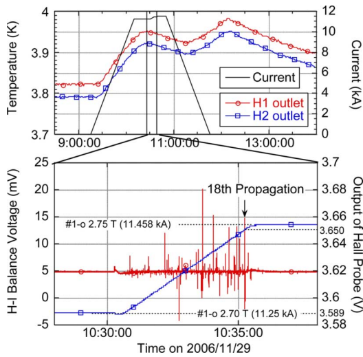
Fig. 5. The outlet temperature, the balance voltage, and the magnetic field at the first excitation to the higher currents on '06/11/29. The 18th propagation of a normal-zone was occurred at #1-o 2.747 T (11.45 kA).
