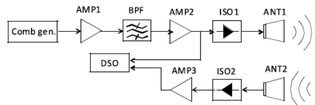
Fig.1: Block diagram of the microwave frequency comb reflectometer.
