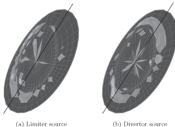
Fig. 2: the \text{H}\alpha emission profile from the atomic hydrogens on cross section 8P. Solid line is the sight of the detector.
