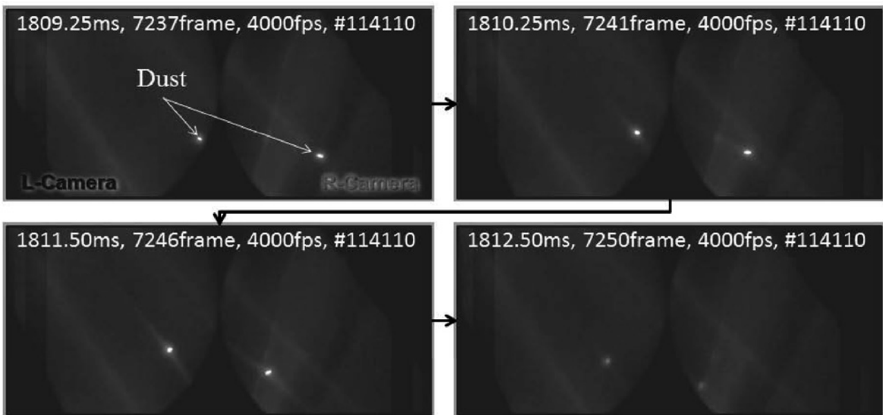
Fig. 1 Four snap shots of movement of a dust observed with a fast framing camera with a stereo-optics for R_{ax}=3.75m .
