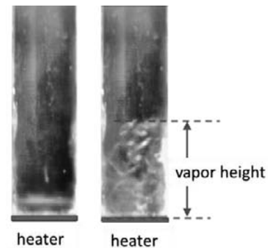
Figure1 Cyclic oscillation inside the rectangular duct in super fluid condition.
