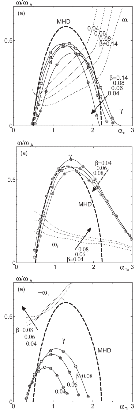
Figure 1: KBM growth rate (lines with marks) and real frequencies (dotted lines), and ideal MHD growth rate (thick dashed lines), which are driven by the density gradient (top), electron temperature gradient (mid), and ion temperature gradient (bottom).
