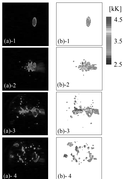
Fig. 2 Abrupt ejection of the Hf droplet from the molten Hf pool as a cathode spot(a-1~4) and the change of surface temperature during the cathode spot instability(b-1~4). Frame interval of each picture from the top to the bottom is 125 \mu s.
