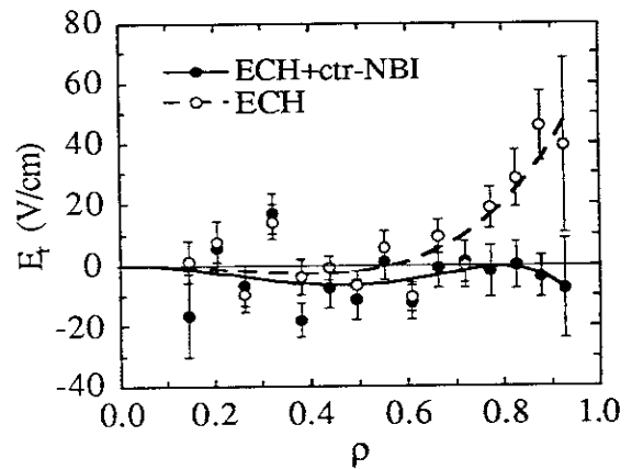
Fig.4 Radial electric field profiles for ECH and for ECH plus ctr-NBI in CHS
