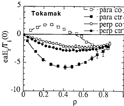
Fig.1 Radial electric field profile in JIPP T-IIU tokamak, where a is plasma minor radius
