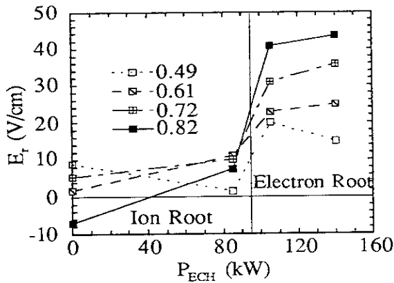
Fig.3 Radial electric field at each averaged minor radius as a function of ECH power in CHS.
