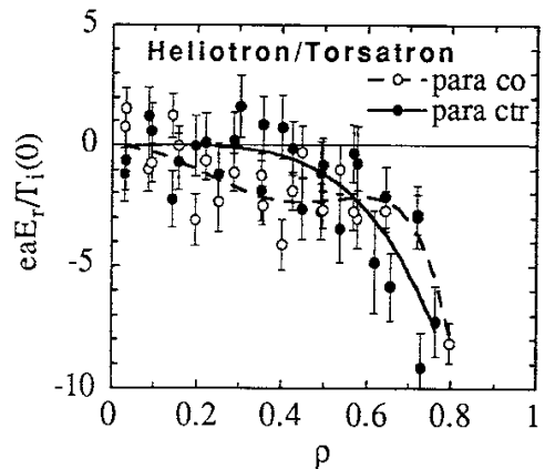
Fig.2 Radial electric field profile in CHS heliotron/torsatron, where a is plasma minor radius.
