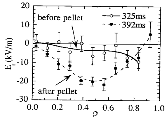
Fig. 5. Radial electric field profiles before and after the pellet injection in heliotron-E.
