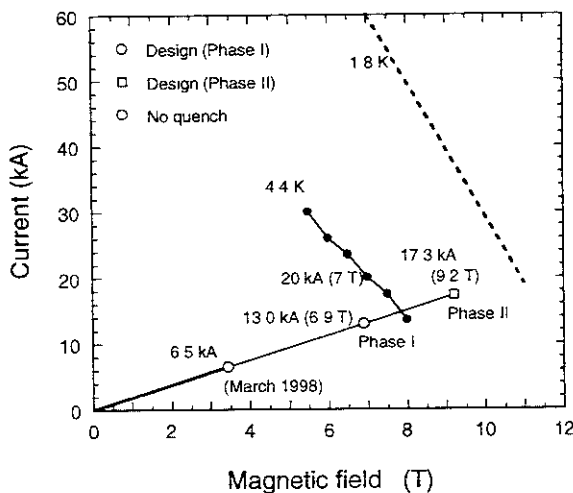
Fig. 8 Performances of Helical Coils for LHD.
