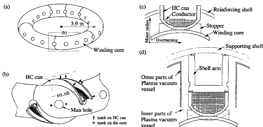
Fig. 5 Manufacturing Process of Helical Coil Package.
