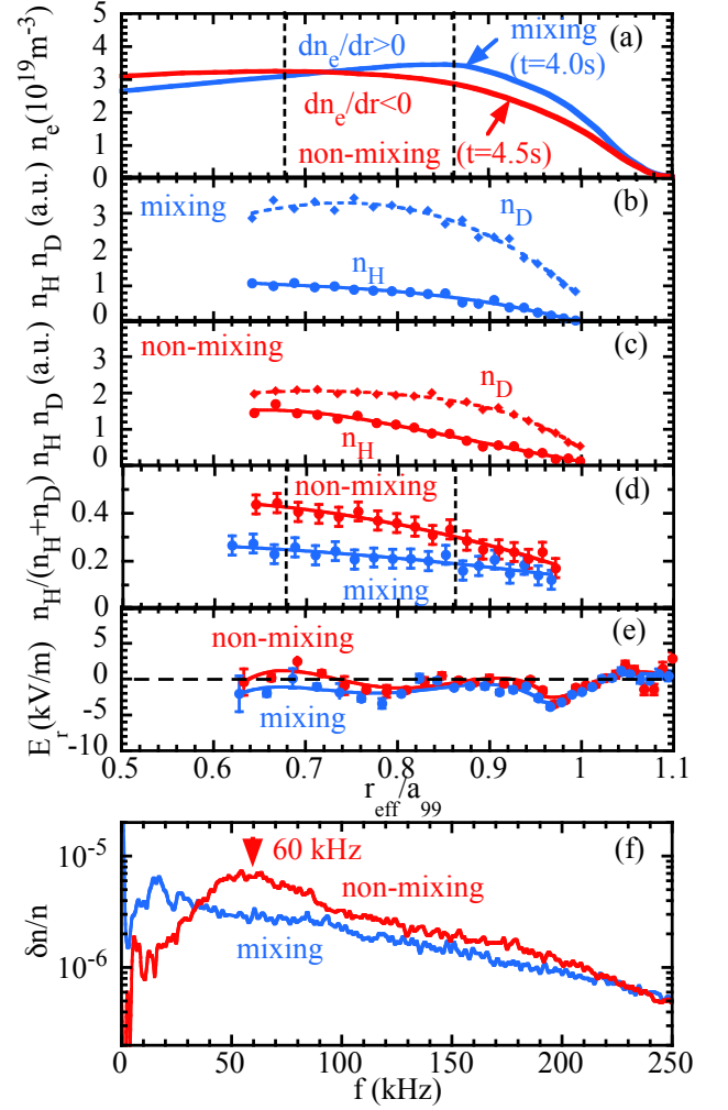
FIG. 6: Radial profiles of (a) electron density, (b)(c) hydrogen and deuterium density, (d) fraction of hydrogen density n_H/(n_H + n_D) , (e) radial electric field, and (f) density fluctuation spectrum at t = 4.0\text{s} in the isotope mixing plasma (#158390) and at t=4.5\text{s} in the non-mixing plasma (#159396) plotted in figure 3.
