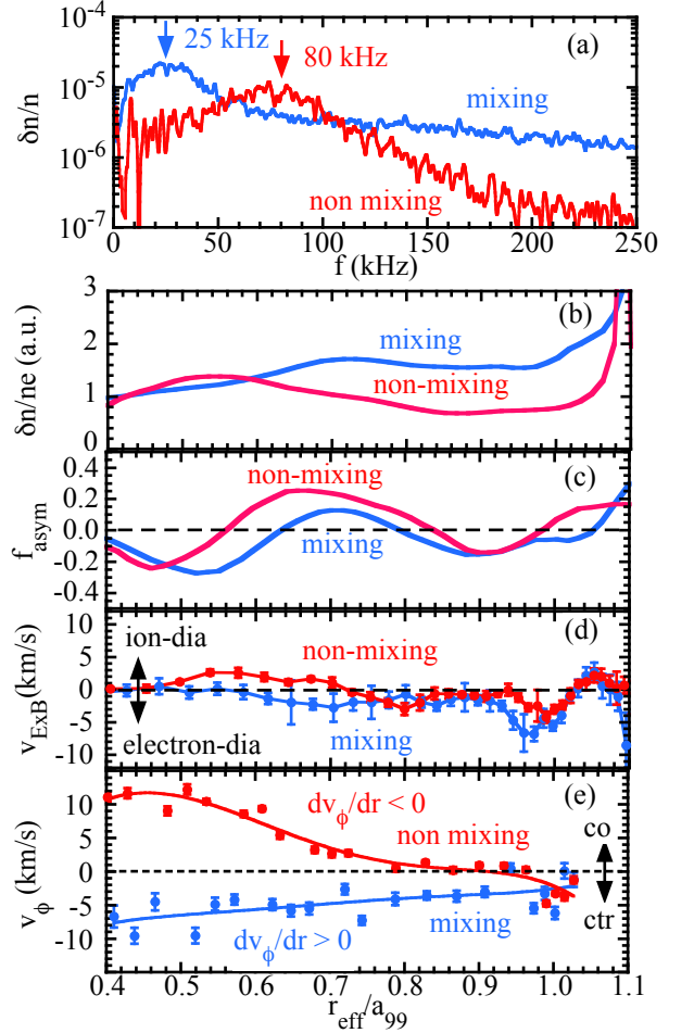
FIG. 2: (a) Density fluctuation spectrum and radial profiles of (b) density fluctuation amplitude, (c) asymmetry factor f_{\text{asym}} of density fluctuation, (d) E \times B velocity, and (e) intrinsic toroidal flow velocity in the isotope mixing (#142325 5.23s) and non-mixing (#142315 3.73s) states in the hydrogen and deuterium mixture plasma with hydrogen beam fueling.
