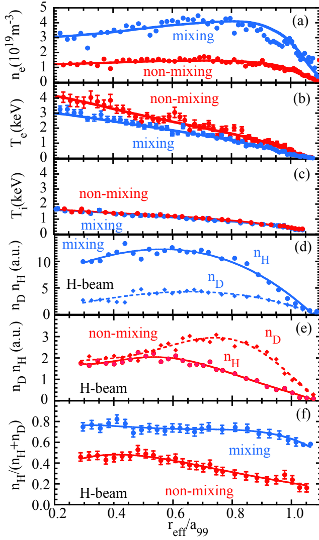
FIG. 1: Radial profiles of (a) electron density, (b) electron temperature, (c) ion temperature, and (d)(e) hydrogen and deuterium density, (f) fraction of hydrogen density n_H/(n_H + n_D) in the isotope mixing (#142325 5.23s) and non-mixing (#142315 3.73s) states in the hydrogen and deuterium mixture plasma with hydrogen beam fueling.
