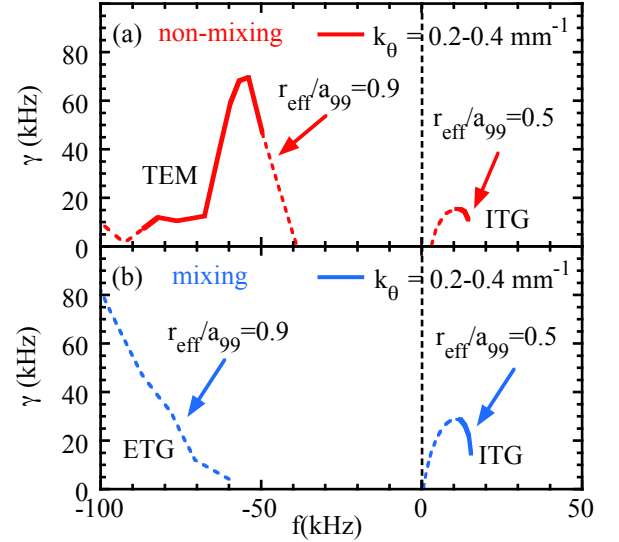
FIG. 3: Linear growth rate at r_{\text{eff}}/a_{99} = 0.5 and 0.9 for the non-mixing (#142315) and isotope-mixing (#142325) states calculated with GKV. The linear growth rates for the wave number of k_{\theta} = 0.2 - 0.4 \text{ mm}^{-1} are indicated with solid line and the dashed lines correspond to the other wave number ( k_{\theta} < 0.2 \text{ mm}^{-1} and k_{\theta} > 0.4 \text{ mm}^{-1} ).
