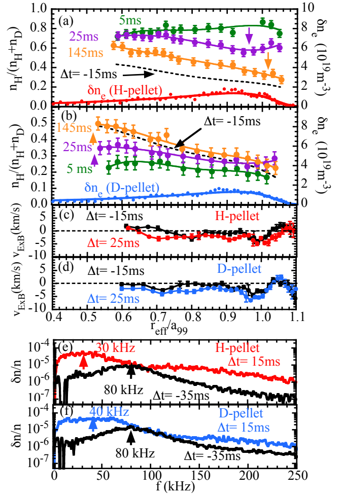
FIG. 8: Radial profiles of (a)(b) fraction of hydrogen density n_H/(n_H+n_D) , and (c)(d) E \times B flow velocity, and (e)(f) density fluctuation spectrum before ( \Delta t < 0 ) and after ( \Delta t > 0 ) (a)(c)(e) the hydrogen (H) pellet injection (#142315) and (b)(d)(f) the deuterium (D) pellet injection (#142314). The radial profiles of the increment of electron density \delta n_e by pellet injection are also plotted.
