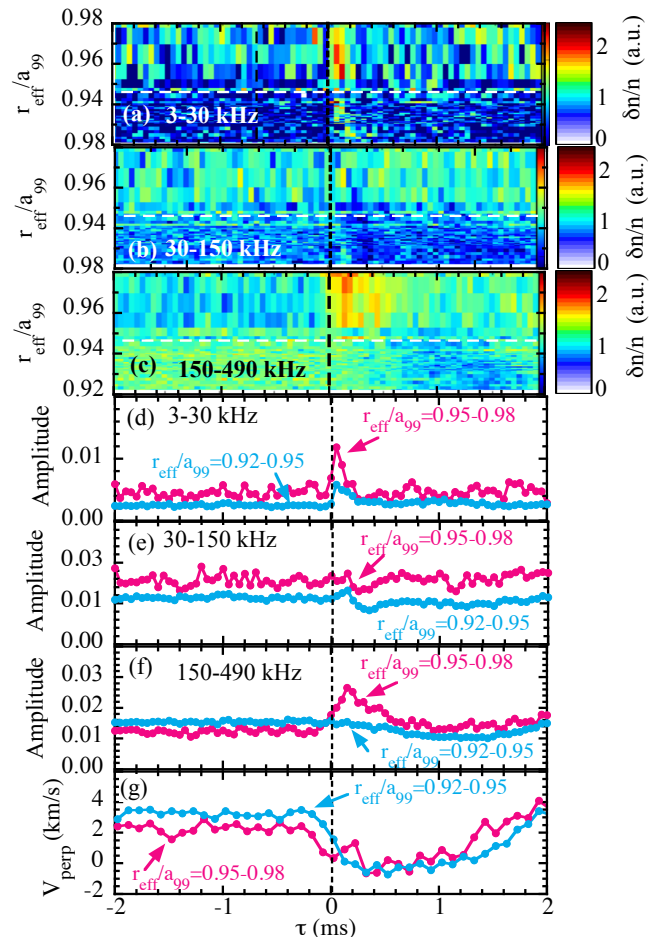
FIG. 3: Contour of density fluctuation in space and in time for (a) low (3 - 30 kHz), (b) middle (30 - 150 kHz), and (c) high (150 - 490 kHz) frequency range at the collapse event ( \tau = 0 ). Time evolution of integrated density fluctuation amplitude for (d) low (3 - 30 kHz), (e) middle (30 - 150 kHz), and (f) high (150 - 490 kHz) frequency range and (g) perpendicular velocity. The horizontal lines are the boundary between the edge region ( r_{\text{eff}}/a_{99} = 0.95 - 0.98 ) and inner region ( r_{\text{eff}}/a_{99} = 0.92 - 0.95 ) of the plasma applied for the plot in Fig. (d)(e)(f)(g).
