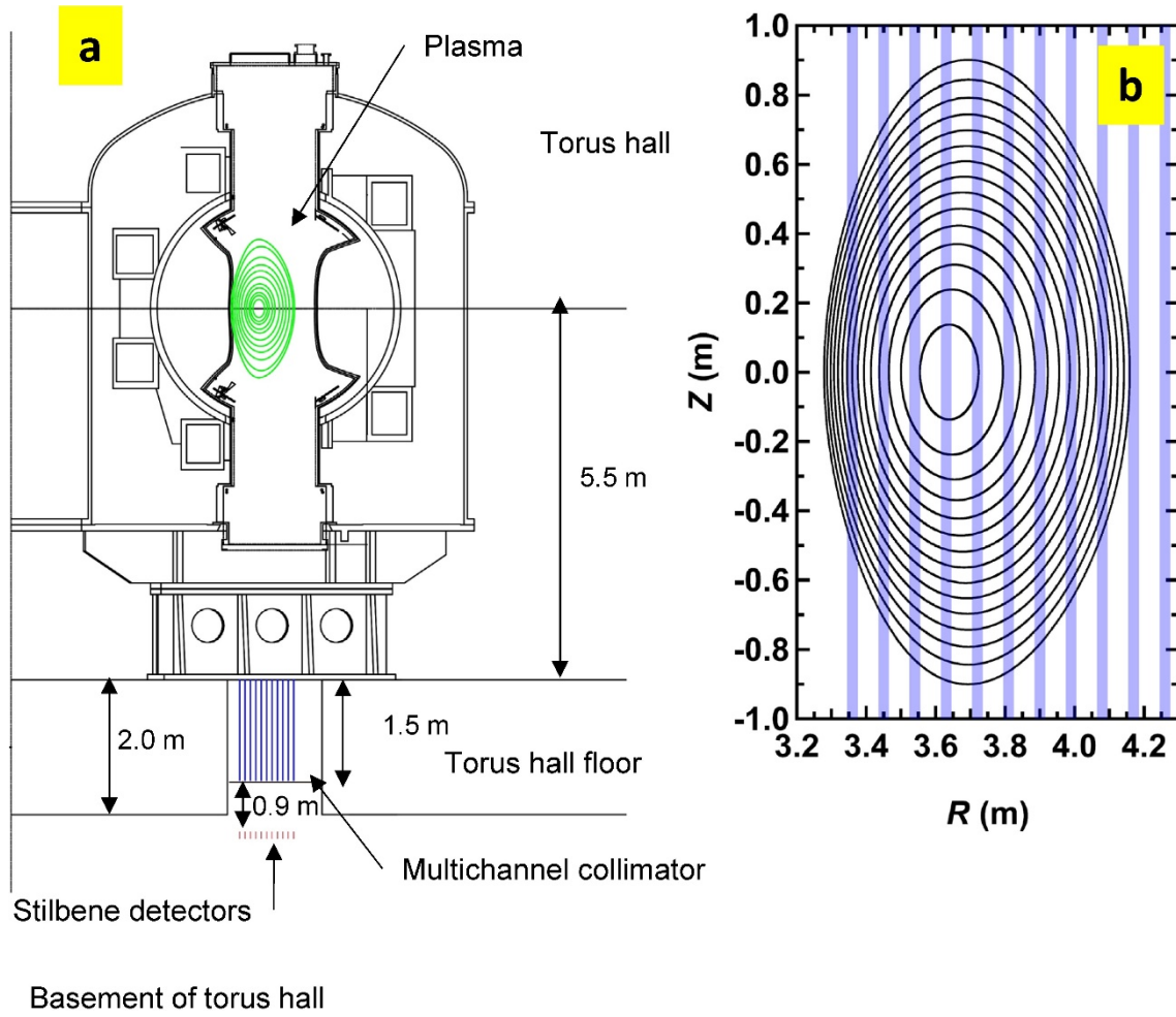
Fig. 2 (a) Schematic drawing of the vertical neutron camera. (b) Sightlines of VNC together with the poloidal cross-section of a plasma.
