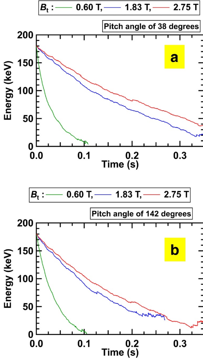
Fig. 11 Time evolution of beam ion energy calculated by DELTA5D code including the collision effect with background plasmas for (a) co-going transit beam ions, (b) counter-going transit beam ions.
