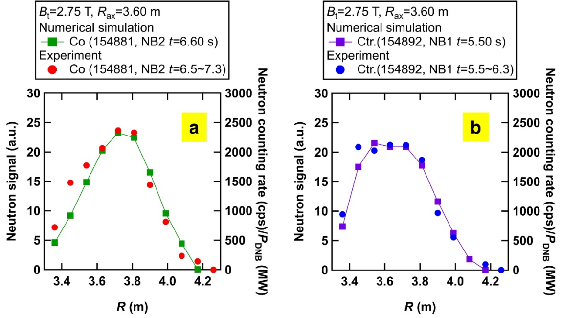
Fig. 13 Line-integrated neutron emission profiles calculated for a high B_t with (a) co-NB injection and (b) ctr.-N-NB injection.
