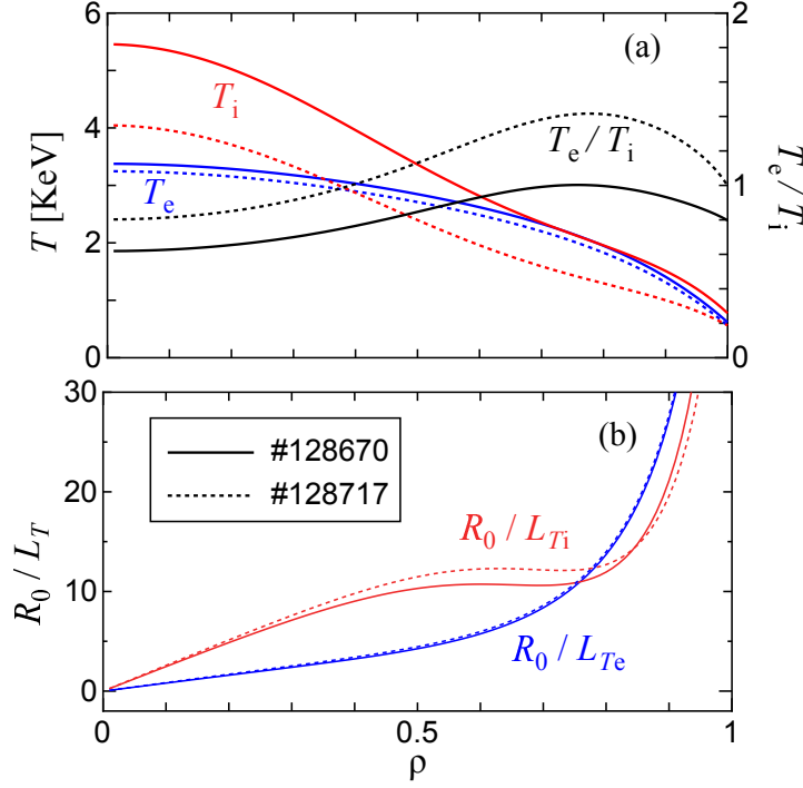
Figure 1. (a) Radial profiles of the temperatures for ions (red curves) and electrons (blue curves), and the temperature ratio T_e/T_i (black curves), and (b) the radial gradient profiles for ion (red) and electron (blue). In both plots, the solid curves represent the results at t = 4.74 s in #128670 (helium-dominated case) and the dotted curves represent that at t = 4.74 s in #128717 (hydrogen-dominated case).
