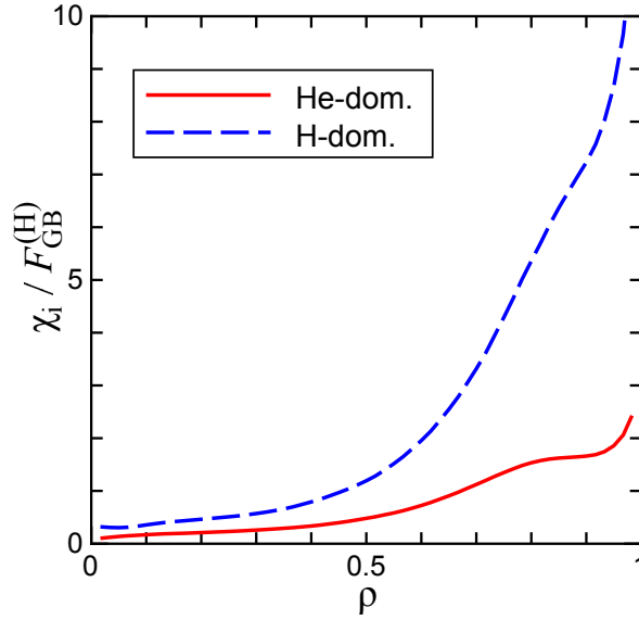
Figure 4. Radial profiles for ion thermal diffusivities estimated by power balance analysis which are normalized by the hydrogen gyro-Bohm factor, F_{GB}^{(H)} \equiv \alpha(\rho_t/R_0)cT_i/Z_H eB .
