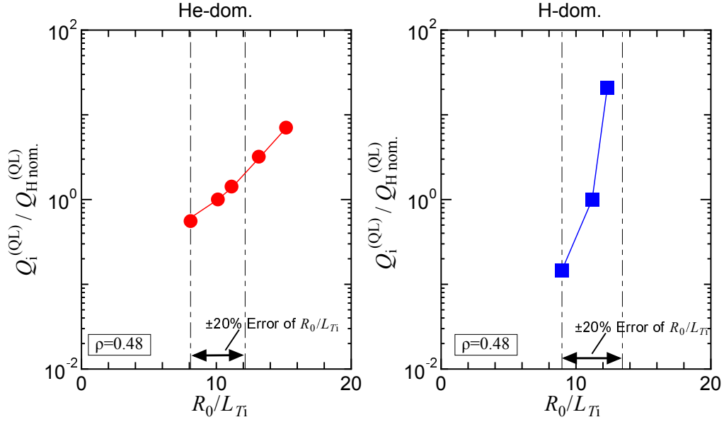
Figure 9. Quasi-linear total ion heat fluxes with changing ion temperature scale lengths in the helium-dominated case (left) and the hydrogen-dominated case (right). Q_i^{(QL)} is normalized by Q_{Hnom}^{(QL)} which is the heat fluxes at the nominal parameters of R_0/L_{T_i} correspond to each case.
