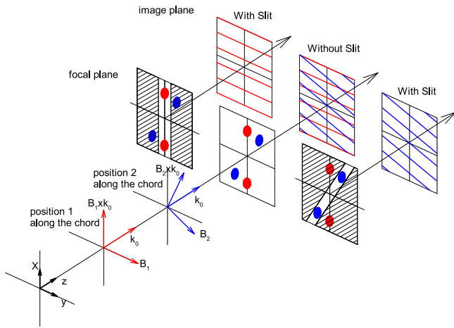
FIG. 1. Principle of magnetic shear technique. k_0 is the wavenumber vector of injected laser beam and B_1, B_2 are the vector of magnetic field at position 1 and 2. Measured wavenumber components are B_1 \times k_0 and B_2 \times k_0 .
