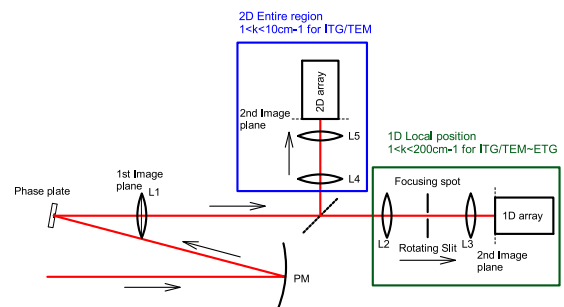
FIG. 3. Detection system.
