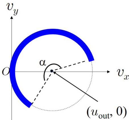
FIG. 4. Schematic diagram of circular-arc-shaped velocity distribution with a central angle \alpha . It is noted that the orbit of each ion is a complete circle.
