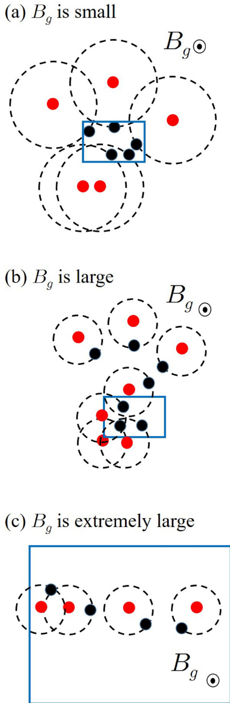
FIG. 5. Schematic diagram of ion gyromotion and a small local area for assembling ion particle information to show velocity distribution in the downstream (a) for small B_g , (b) for large B_g , and (c) for extremely large B_g . The black and red circles indicate the actual positions of ions and the guiding center positions of the ions, respectively, and the dashed lines denote gyromotion orbits. The blue boxes represent small local areas.
