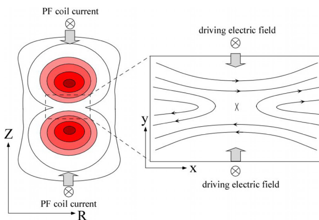
FIG. 1. Schematic diagram of our simulation model. The left panel shows merging torus plasmas. The right panel is the area computed by a particle simulation with the PASMO code.
