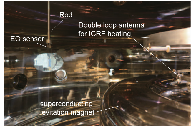
FIG. 8. The EO sensor mounted inside the supporting rod is inserted from the top port. The vacuum vessel of RT-1 contains the levitation superconducting magnet and the double-loop antenna for ICRF heating.
