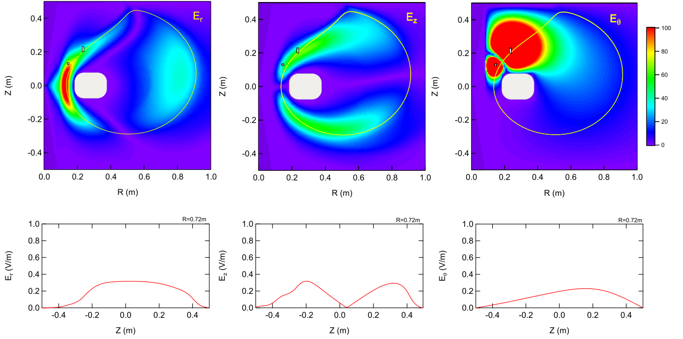
FIG. 13. Two-dimensional profiles of the electric fields excited by the double-loop antenna in RT-1. The current densities in the upper and lower loops are set to J_{ext} = +252 A and -252 A, respectively. Bottom panels show the profiles of E_r , E_z , and E_\theta along the line R = 0.72 m in RT-1, plotted from the corresponding 2D profiles.
