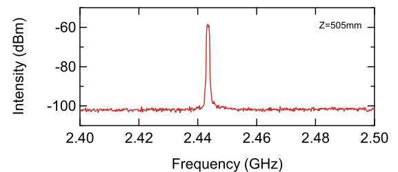
(b) Spectrum of EC wave measured by the EO sensor
