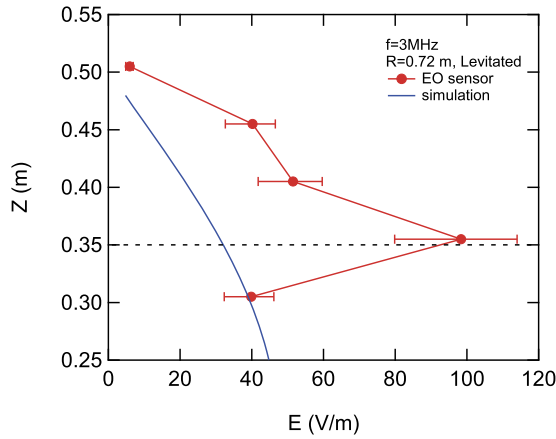
FIG. 10. E_0 (closed circles) vertically measured by the EO sensor along R = 0.72 m in helium plasma. The ICRF power is 7 kW. The separatrix (dashed line) is located at (R, Z) = (0.72 \text{ m}, 0.35 \text{ m}) . The input parameter for the simulation was the measured antenna current (252 A).
