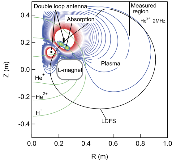
FIG. 9. Contours of the electric field E_0 excited by the double-loop antenna in helium plasma. L-magnet indicates the levitation magnet. The antennas are located outside the LCFS. The contours of the power absorption area for \text{He}^{2+} are also plotted. The ion cyclotron layers for \text{H}^+ , \text{He}^{2+} , and \text{He}^+ are depicted.
