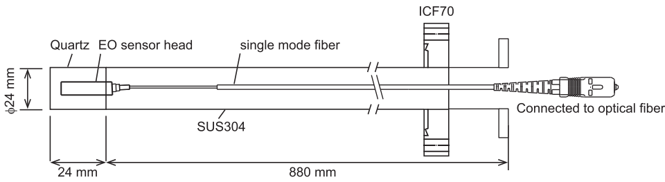
FIG. 2. Schematic of the EO sensor mounted in a shaft for inserting into RT-1 plasmas. To measure the spatial profile, the shaft is mounted on a motor drive system at the flange.
