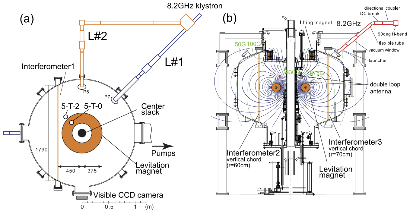
FIG. 4. Magnetosphere plasma device RT-1. (a) Top view and (b) cross sectional view. For the electric field measurements, the EO sensor head was inserted from the 5-T-0 ( R = 0.245 m) and 5-T-2 ( R = 0.72 m) ports. The double-loop antenna for ICRF heating is mounted on the center stack.
