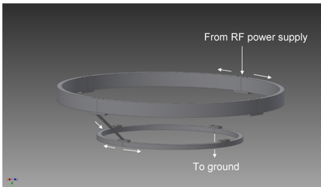
FIG. 5. Double-loop antenna and RF current flow for ICRF heating in RT-1.
