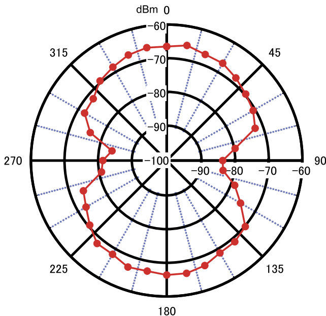
FIG. 3. Radiation pattern of the EO sensor acquired at 3 MHz.
