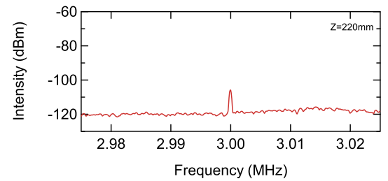
(a) Spectrum of ICRF wave measured by the EO sensor
