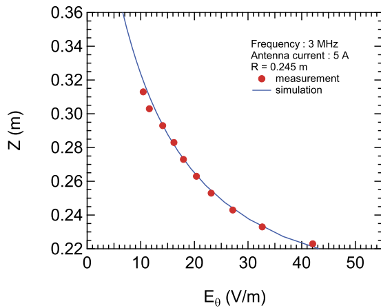
FIG. 7. Electric field profile of E_0 at 3 MHz measured by the EO sensor (closed circles) in RT-1 in the air experiments. The simulation result (blue curve) is also plotted.
