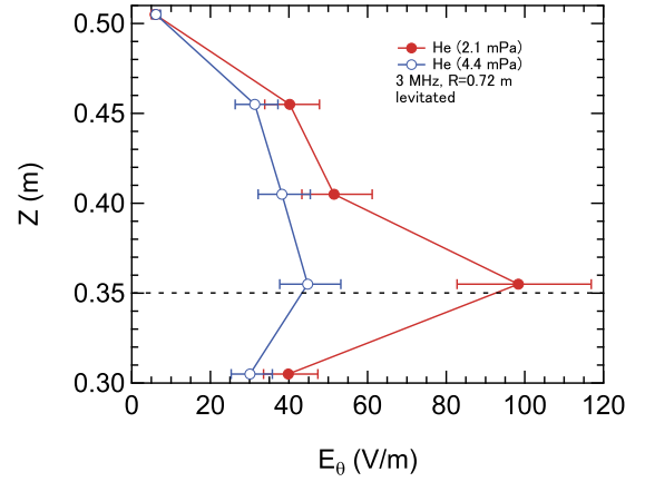
FIG. 11. E_0 measured by the EO sensor in helium plasmas. The helium gas pressures were 2.1 mPa (closed circles) and 4.4 mPa (open circles).
