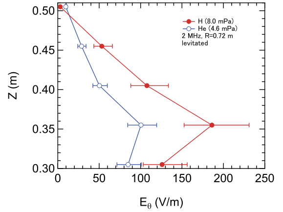
FIG. 12. E_0 measured by the EO sensor in plasmas. The fill gas pressures are mixed hydrogen at 8.0 mPa and helium at 0.6 mPa (closed circles) and helium at 4.6 mPa (open circles).
