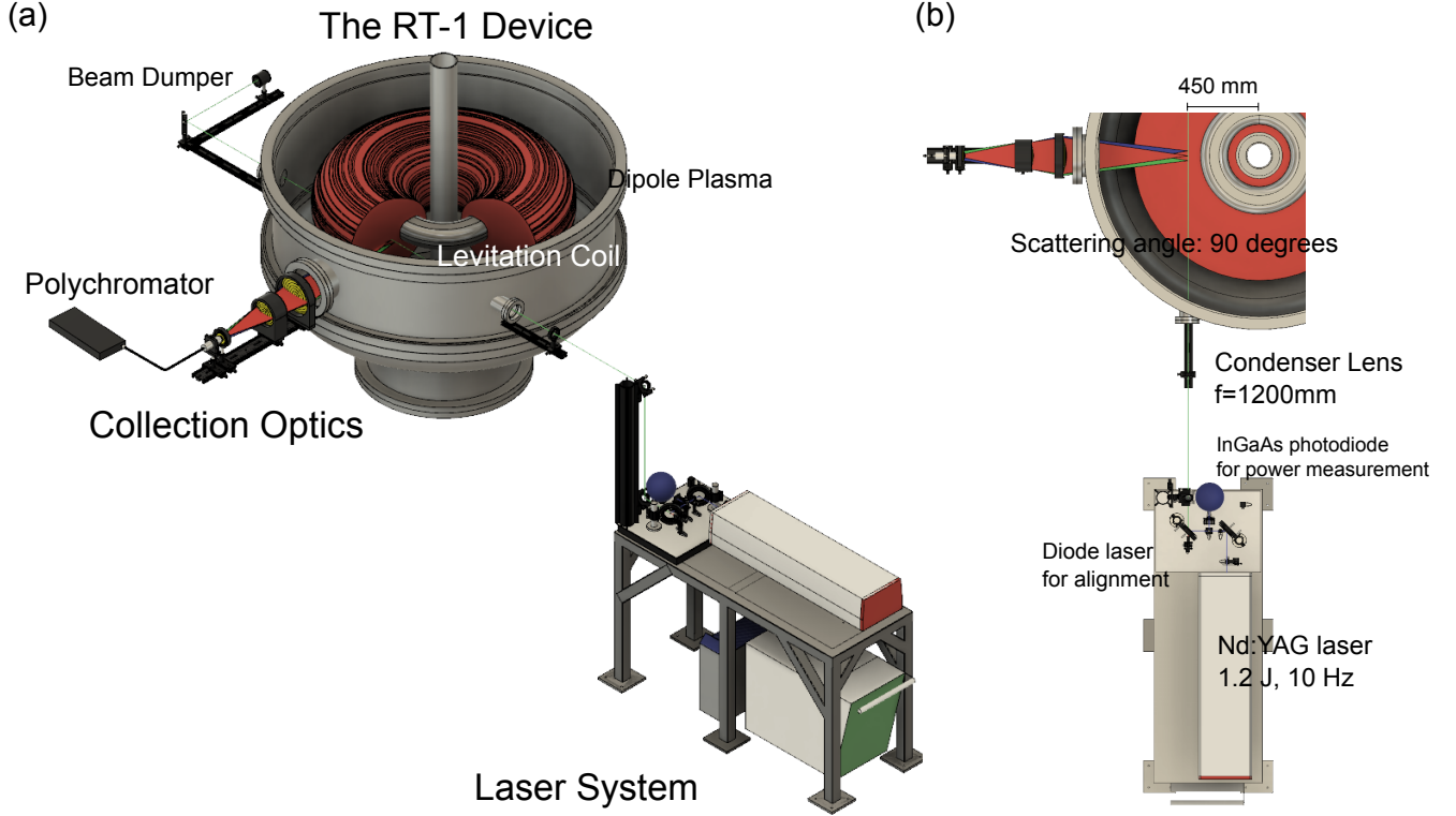
FIG. 1. (a) Overview and (b) sideview of the TS system in the RT-1 device.
