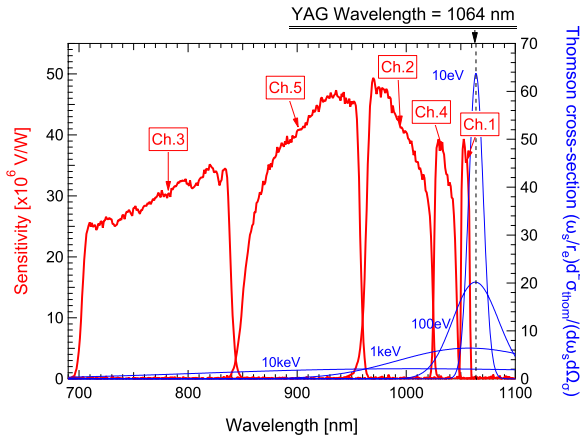
FIG. 4. Spectral sensitivity of the polychromator filters (red) and the spectrums of the Thomson cross section (blue).
