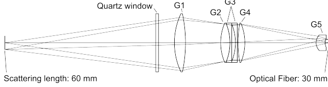
FIG. 2. The set of collection optics lenses. The G1, G2, G4, and G5 lenses are convex, and the two G3 lenses are concave.
