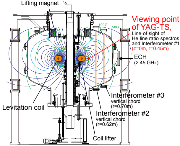
FIG. 7. Cross-sectional view of the RT-1 magnetospheric plasma device.
