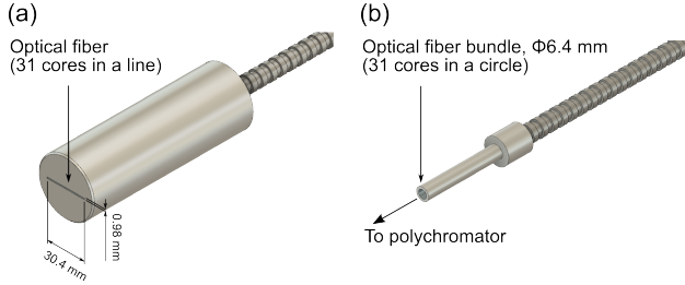
FIG. 3. Schematic of the optical fiber bundle: (a) optical fiber on the input side of the scattered light and (b) the optical fiber bundle on the output side, which is inserted into the polychromator.
