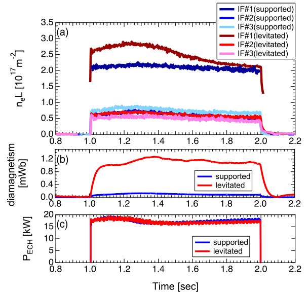
FIG. 8. Time evolution of (a) the line-integrated electron density, (b) the diamagnetism, and (c) the injection power of ECH in the coil-supported and coil-levitated cases.
