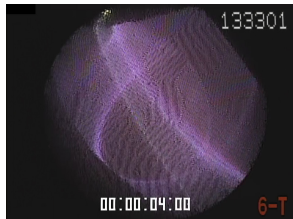
Figure 9 The first light of LHD deuterium plasma on March 7, 2017 (#133301).
