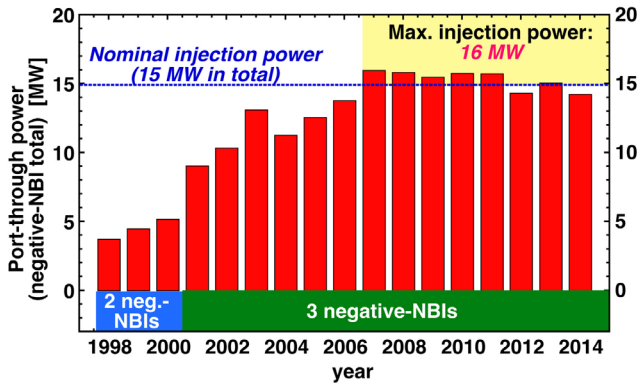
Figure 4 Progress of total port-through beam power obtained with two NBI systems (1998-2000) and three of them (2001-2014). The maximum port-through power of 16 MW was achieved in 2007 and more than 15 MW of the port-through power was obtained several years after the achievement.
