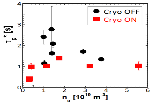
Figure 7 Global particle confinement time ( \tau_p^* ) for various density regime for cases with cryo-sorption pumping OFF (●) and ON (■).
