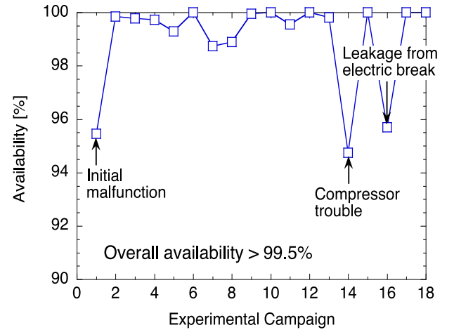
Figure 2 Availability of the LHD cryogenic system.
