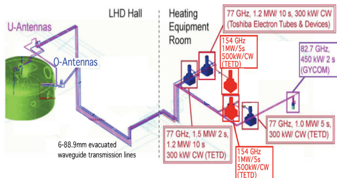
Figure 5 Present configuration of the ECH system in LHD. (cited, Fig. 2 in Ref. [29].)
