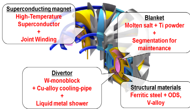
Figure 10 Innovative engineering ideas to realize the helical fusion reactor FFHR-d1.
