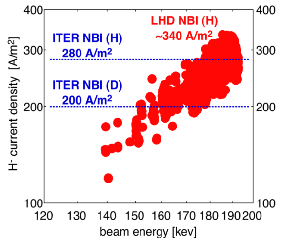
Figure 3 H^- current density obtained with the new beam accelerator as a function of beam energy.
