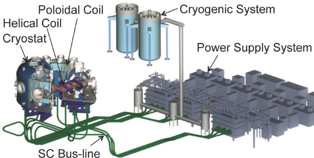
Figure 1 Superconducting system of LHD (cited, Fig. 1 in Ref. [8]).
