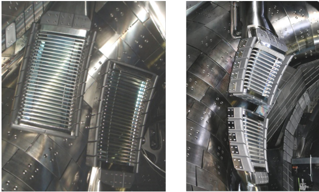
Figure 6 Two kinds of ICRF antennae in the LHD. Left picture shows a hand shake type antenna (HAS), and right pictures shows a field-aligned impedance transforming antenna (FAIT).
