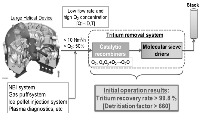
Figure 8 Schematic diagram of tritium removal system: the tritium removal system treats all exhaust gas from LHD and the auxiliary system.
