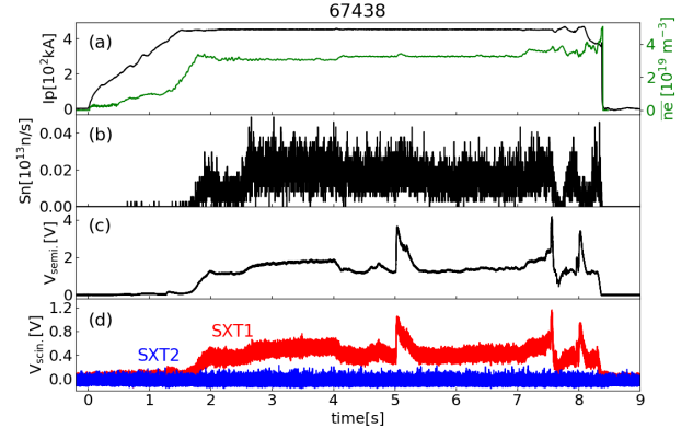
FIG. 2. Signals of (a) the plasma current and the line averaged electron density measured by the HCN interferometer, (b) the total neutron emission rate obtained with fission chamber, (c) semiconductor-based SX diagnostic 13 , and (d) scintillator-based SX diagnostic are shown.
