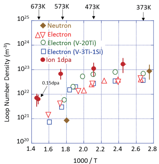
Fig. 6 Temperature dependence of dislocation loop number density. Data by electron irradiation for V-4Cr-4Ti (0.8~1.3 × 10 -2 dpa/s) [6] and V-20Ti and V-3Ti-1Si (1.6 × 10 -4 dpa/s) [4] are also shown for comparison.
