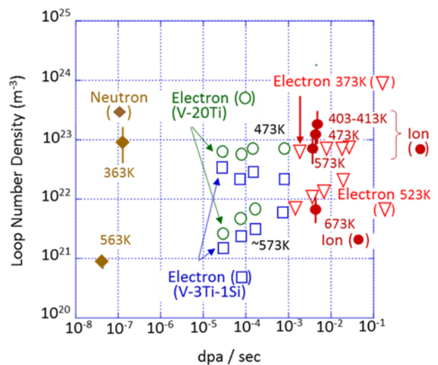
Fig. 7 Damage rate dependence of dislocation loop number density. Data by electron irradiation for V-4Cr-4Ti at 373 K and 523 K [6] and V-20Ti and V-3Ti-1Si at 473 K and ~573 K [4] are also shown for comparison.
