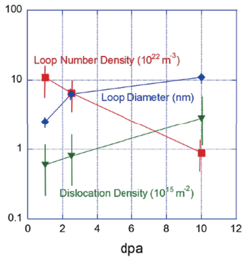
Fig. 4 Microstructural parameters as a function of dose (dpa) by 2.4 MeV Cu 2+ ion irradiation at 473 K.
