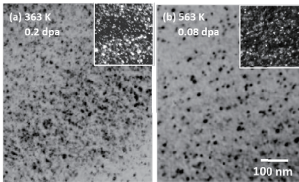
Fig. 5 Microstructural evolution by neutron irradiation. (a) Irradiation in BR2. (b) Irradiation in JMTR. Upper right corners show WBDF images.
