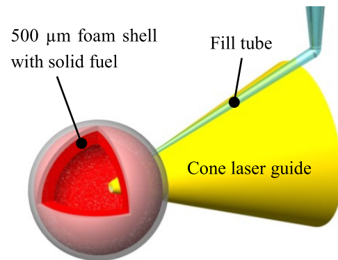
Fig. 1 Typical appearance of FIERX foam shell target. A cone guide and a fill tube are attached to a foam shell. The shell diameter is 500\ \mu\text{m} . A uniform solid fuel has to be formed within the foam layer of a \sim 20\ \mu\text{m} thickness. The sphericity is required to be more than 99%.
