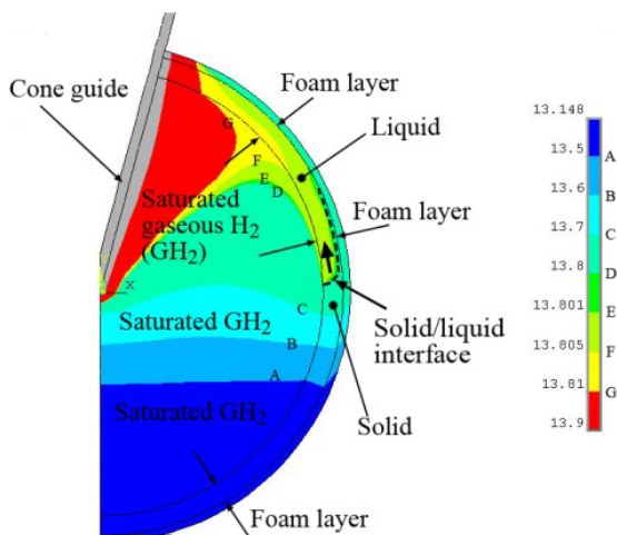
Fig. 3 Successful simulation of solidification control in the 500 μm FIREX target [7]. The figure represents temperature distribution in the foam shell 8800 sec after the start of the calculation. The solid/liquid interface is moving upward in the foam layer.
