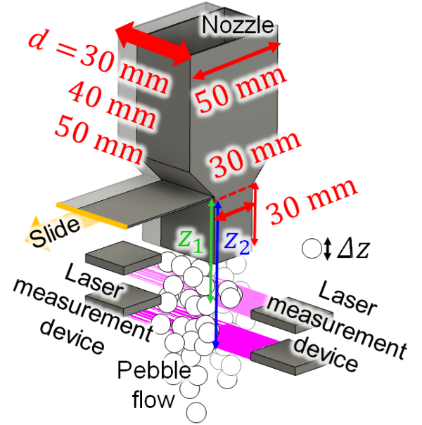
Figure 2 The experimental system of the shielding rate of the pebble flow.
