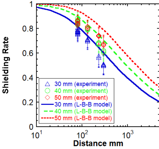
Figure 3 Experimental results of the shielding rate by the pebble flow ( \triangle : d = 30 mm, \circ : d = 40 mm, \diamond : d = 50 mm). The equation of the shielding rate model (solid line : d = 30 mm, long broken line : d = 40 mm, broken line : d = 50 mm).
