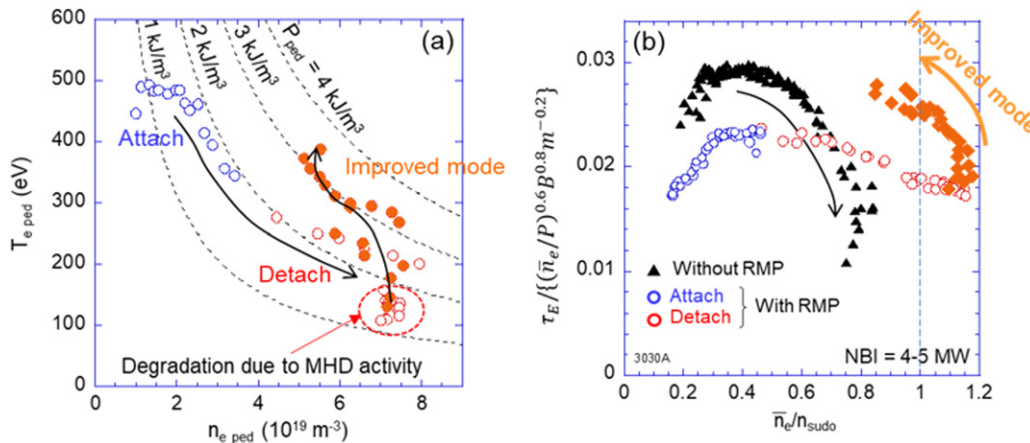
Figure 7. (a) Evolution of n_{\text{eped}} and T_{\text{eped}} at pedestal top during the discharge with RMP, (b) energy confinement time scaled with gyro-Bohm scaling as a function of line-averaged density, which is normalized with density limit. Blue circles: attached phase with RMP, red circles: detached phase with RMP, orange diamonds: improved mode with RMP (detach), black triangles: without RMP. (Data from deuterium plasmas.)
