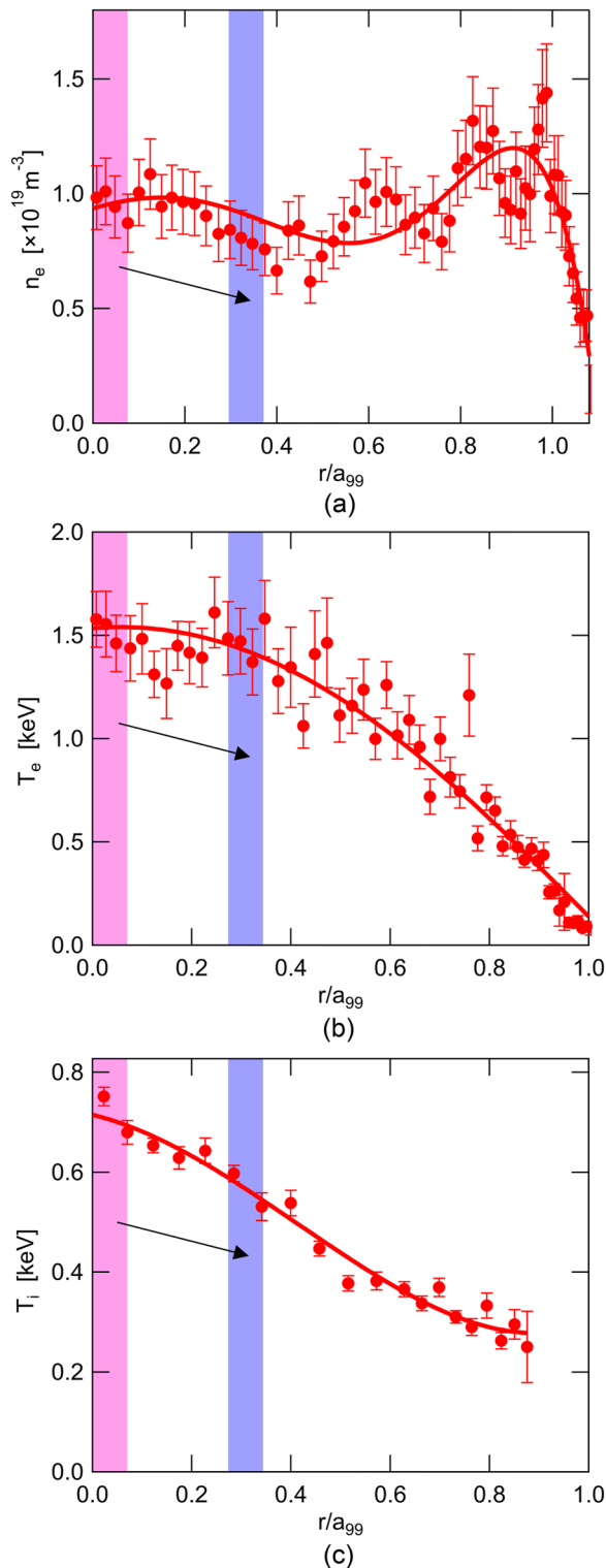
FIG. 10. (a) Electron density and (b) electron temperature from TS at t = 5.113 s and (c) ion temperature from CXRS at t = 5.1225 s for LHD shot No. 164450.
