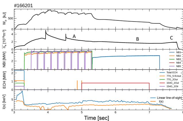
FIG. 4. Discharge waveforms for LHD shot No. 166201. The ECE signal, with a straight viewing chord at channel 5, and I(s) , calculated using the raytracing code with the TS data, are plotted in the bottom panel.
