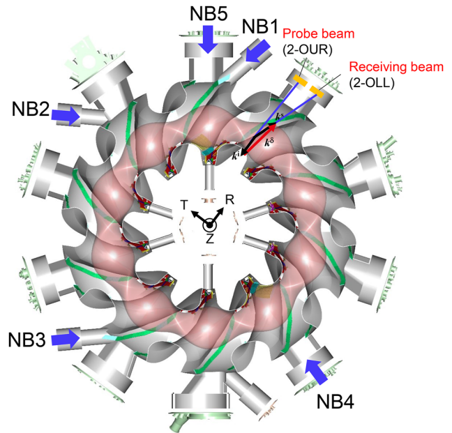
FIG. 1. Top view of LHD. The probe and the receive beams are located at the 2-OUR and 2-OLL ports, respectively. The wavevectors are scaled to understand the geometry.
