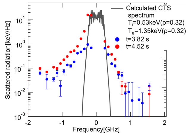
FIG. 11. CTS spectra at t = 3.82 and 4.52 s for LHD shot No. 164450. The theoretical CTS spectrum for bulk ions in black is calculated using data from TS and CXRS. The fast ion component is not included in the CTS spectrum. The negative and positive frequencies correspond to Co-NB2 and counter-NB1 directions, respectively.
