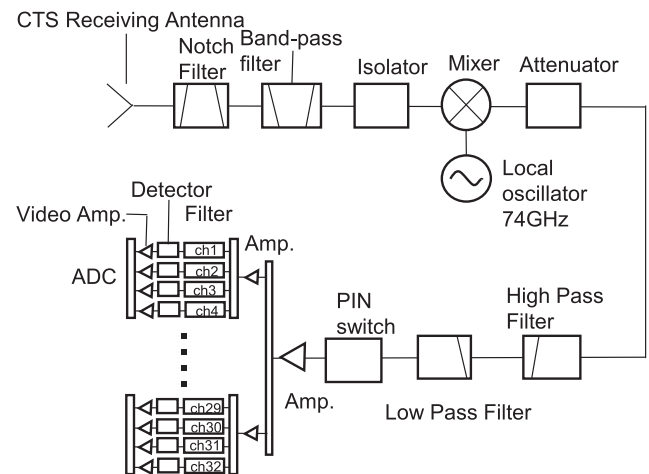
FIG. 2. Schematic diagram of the CTS receiver.
