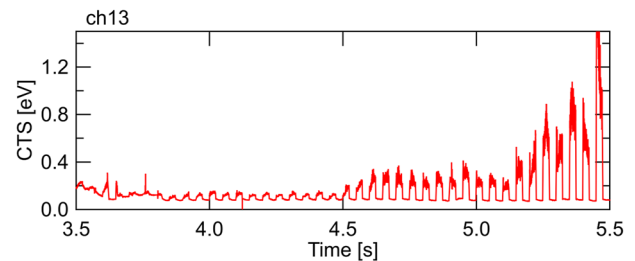
FIG. 9. Receiver signal of channel 13, containing scattered radiation and background ECE in LHD shot No. 164450.
