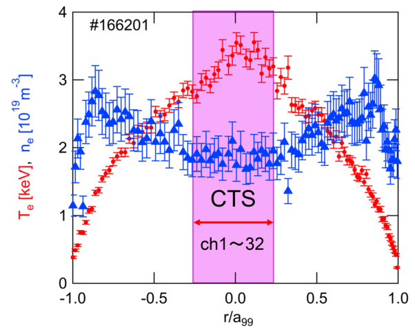
FIG. 5. Electron temperature and density profiles at t = 5.0 s for LHD shot No. 166201. The CTS receiver channels cover the hatched area.
