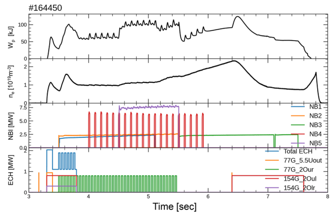
FIG. 8. Discharge waveforms for LHD shot No. 164450.
