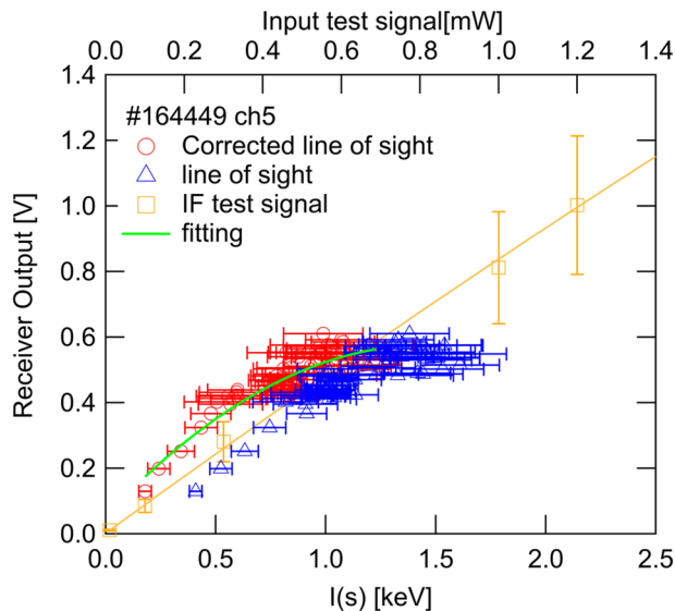
FIG. 7. ECE signal measured by channel 5 of the CTS receiver during CTS measurement. Triangles represent T_e calibrated by ECE and TS measurements. Open circles correspond to I(s) after raytracing correction. The output signal (squares) is the same as that in Fig. 6.
