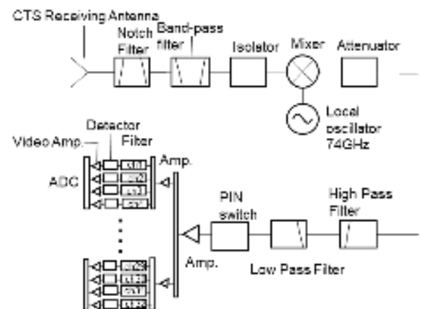
FIG. 2. Schematic diagram of the CTS receiver.
