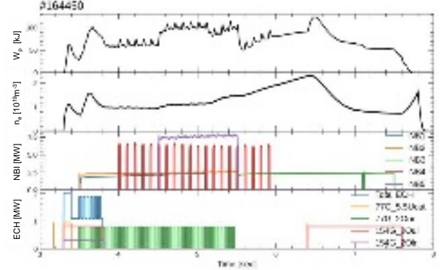
FIG. 8. Discharge waveforms for LHD shot#164450.
