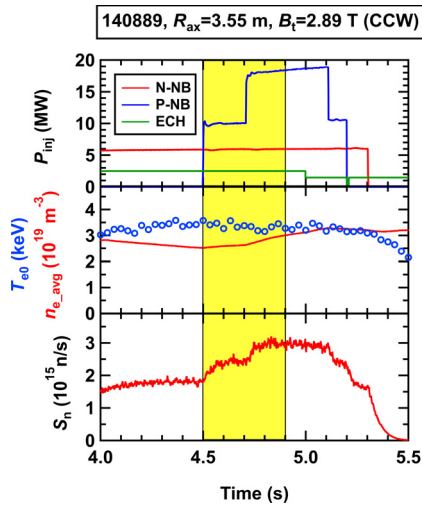
Fig. 1 Typical time evolution of deuterium plasma discharge. Yellow region fulfills the general restrictions in this analysis.
