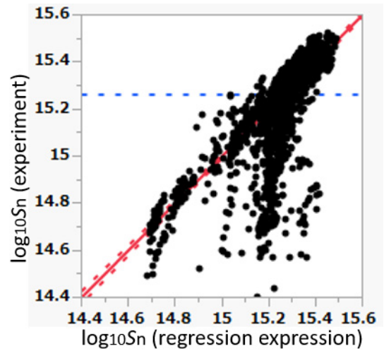
Fig. 2 Comparison of \log_{10} S_n values between the experimental measurement (vertical axis) and ones based on the regression expression (horizontal axis).
