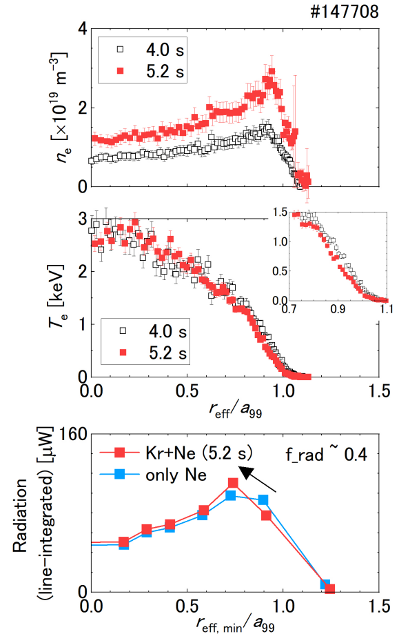
Fig. 7 After Kr+Ne seeding, T_e locally decreased at |r_{\text{eff}}/a_{99}| > 0.8 while the n_e profile shape was not changed. The radiation region moved upstream with the suppression of impurity accumulation toward the central plasma compared with the same f_{\text{rad}} using Ne only seeding.
