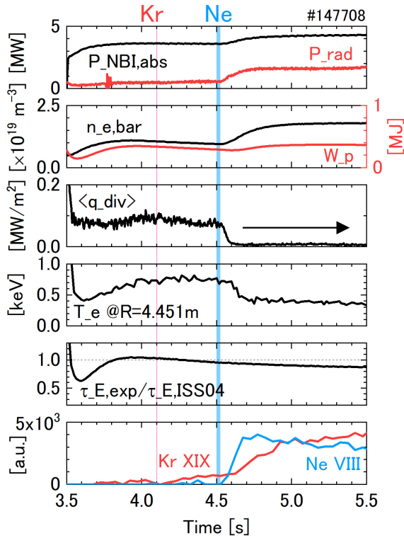
Fig. 6 Divertor detachment using Kr+Ne superimposed seeding. f_{\text{rad}} \sim 40\% and 90\% decreased \langle q_{\text{div}} \rangle were sustained for \sim 1 s. \tau_{\text{E,exp}}/\tau_{\text{E,ISS04}} was 10% higher than the Ne only seeding case. Pre-seeded Kr emission was drastically enhanced after Ne seeding.
