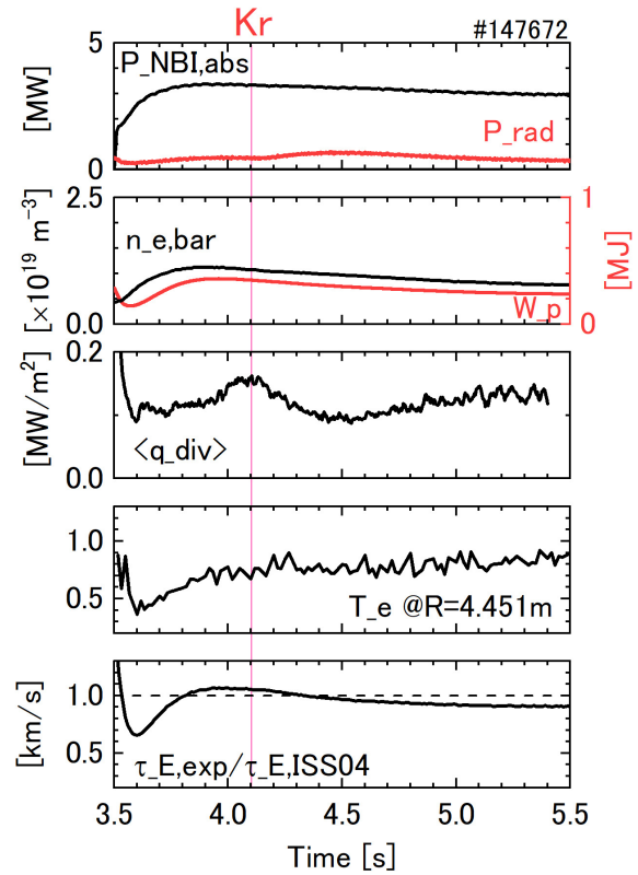
Fig. 5 Divertor detachment using Kr seeding. Plasma response was much slower than the case of only Ne seeding. The maximum f_{\text{rad}} \sim 21\% was observed at 4.5 s. Here, \langle q_{\text{div}} \rangle gradually decreased by \sim 43\% but reduction of edge T_e was not observed. \tau_{E,\text{exp}}/\tau_{E,\text{ISS04}} is > 0.9 .
