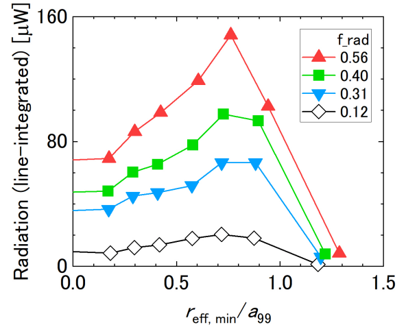
Fig. 2 f_{rad} dependence of radiation profile. Radiation was enhanced at upstream region ( r_{eff,min}/a_{99} \sim 0.8 ) with increase of f_{rad} .
