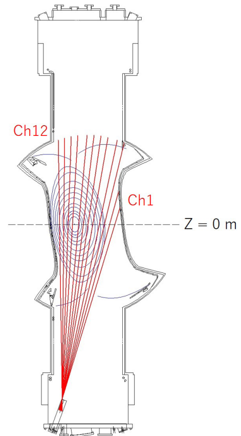
Fig. 3 Sightlines of resistive bolometer arrays.
