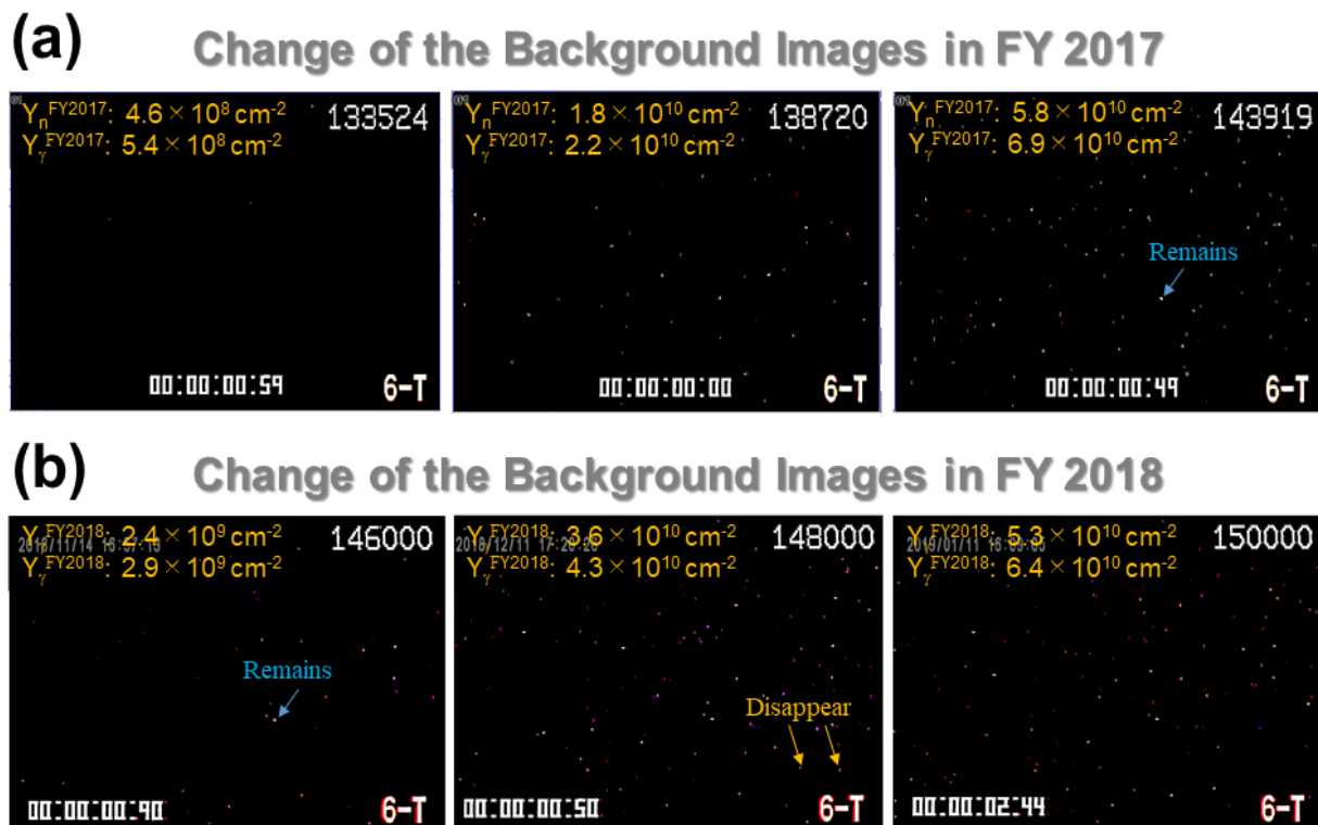
Fig. 7 The change of the background images taken before the ignition of the plasma discharges as the cumulative radiation fluxes in the two experimental campaigns (FY 2017 and FY 2018), respectively.
