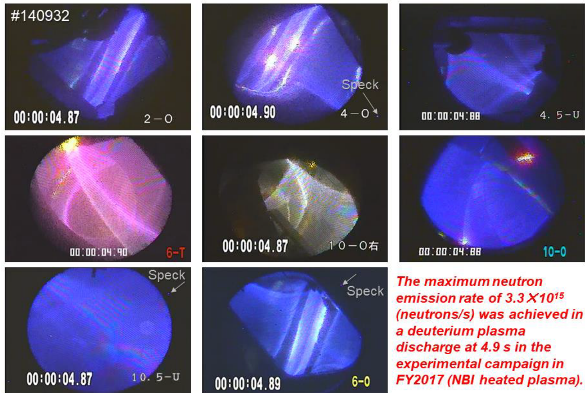
Fig. 6 Plasma images taken with the radiation resistant camera systems at the time of the maximum neutron emission rate in a deuterium plasma discharge in FY 2017.
