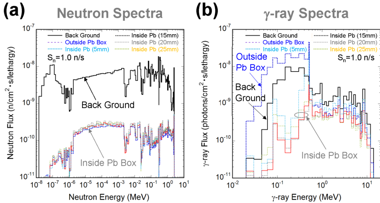
Fig. 5 (a) The calculated neutron spectra at the shield box, and (b) the calculated gamma-ray spectra at the shield box. The solid black lines represent the background spectra. The colored dotted lines present the spectra in the lead box with various thicknesses of the lead plates. The blue broken lines indicates the spectra at a space between polyethylene blocks and the lead box.
