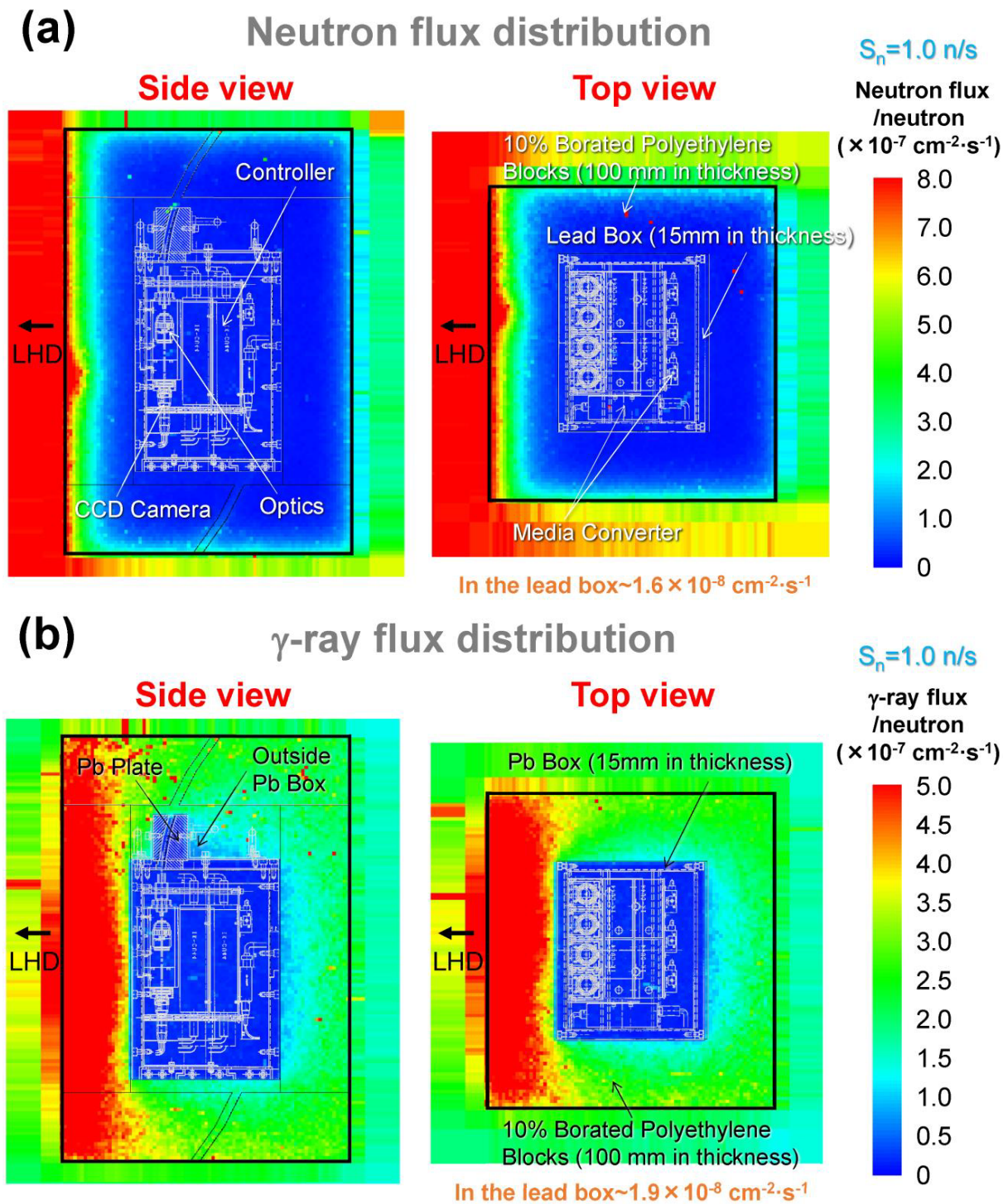
Fig. 4 The simulation of the side and top cross-section of (a) the neutron and (b) the gamma-ray flux distribution in the shield box #2.
