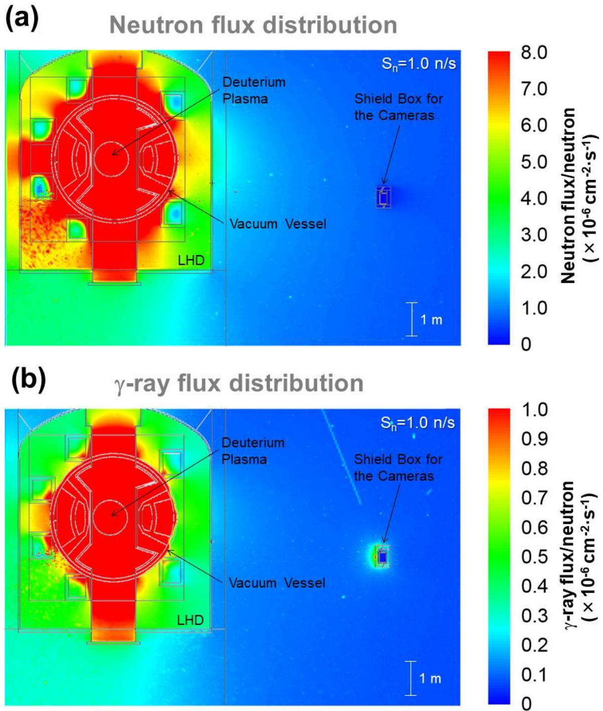
Fig. 3 The simulation of the vertical cross-section of (a) the neutron and (b) the gamma-ray flux distribution in the torus hall for a neutron emission rate of 1.0 n/s in the LHD deuterium plasma.
