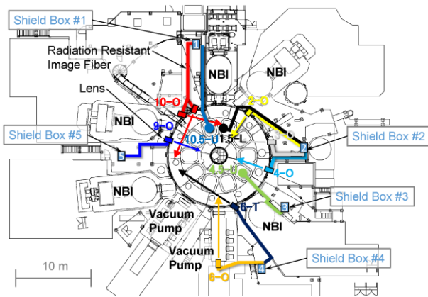
Fig. 1 The top view of the setup of the radiation resistant camera system for monitoring deuterium plasmas in LHD.
