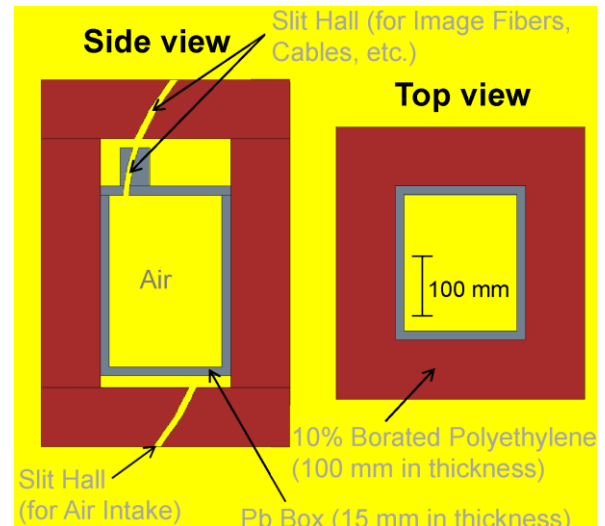
Fig. 2 The side and top cross-sectional view of the three-dimensional model of the shield box for the MCNP code.
