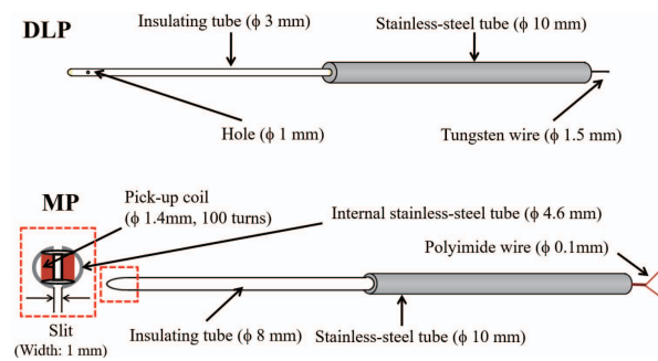
Fig. 2 Schematic drawings of DLP and MP.
