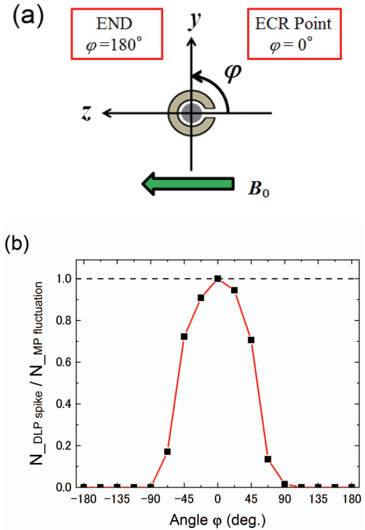
Fig. 6 (a) Cross-sectional view of DLP and coordinate system. \varphi is the angle of normal vector of probe surface with respect to z -axis. \varphi = 0 is set to upstream direction. (b) Angle dependence of the ratio of number of large amplitude negative spikes in DLP signal ( N_{\text{DLP spike}} ) to the number of large amplitude magnetic fluctuations ( N_{\text{MP fluctuation}} ).
