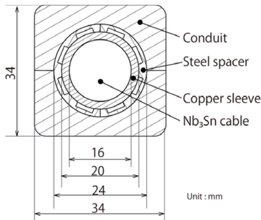
Fig. 3 Cross-section of the joint sample at the butt joint.
