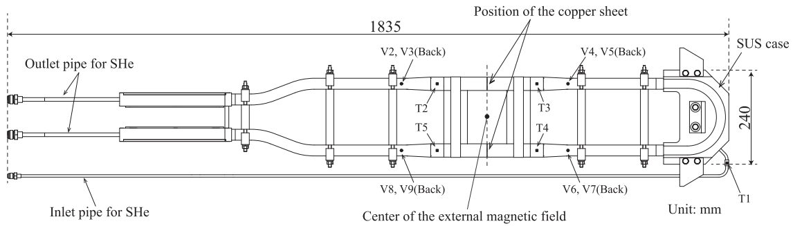
Fig. 1 Schematic view of the joint sample. V2-V9 and T1-T5 indicate the position of the voltage taps and thermometer, respectively.
