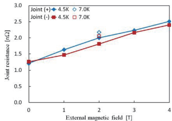
Fig. 4 Joint resistance of the joint samples.
