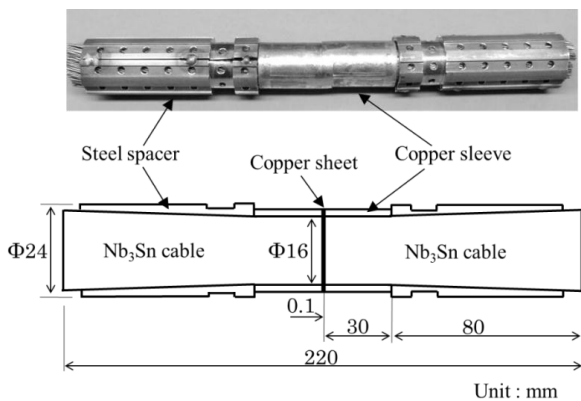
Fig. 2 Photograph and configuration of the butt joint without conduit.
