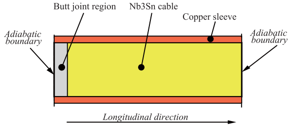
Fig. 5 Schematic view of the numerical model simplifying half of the butt joint.
