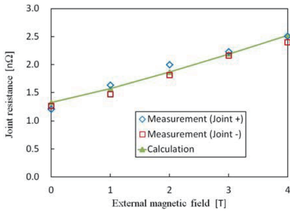
Fig. 6 Comparison between measurement and calculation with regard to joint resistance at 4.5 K.
