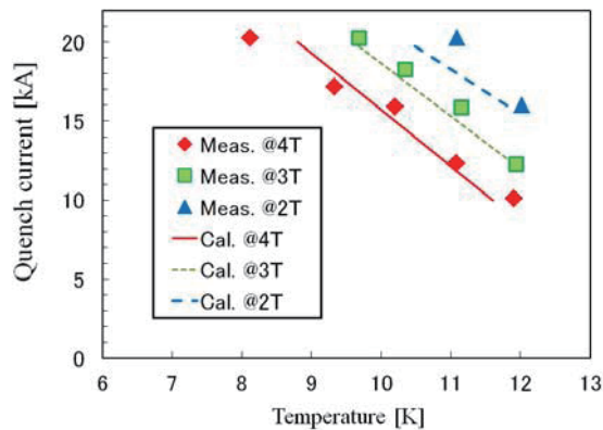
Fig. 7 Comparison between measurement and calculation with regard to quench current.
