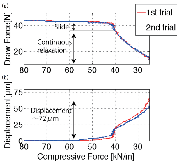
Fig. 5 Typical waveforms draw force along relaxation of compressive force. (b) Typical waveforms of strand displacement along relaxation of compressive force. A slip of 3 μm is observed at a press load of approximately 40 kN/m.
