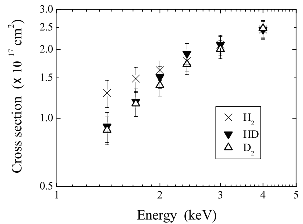
Fig. 5 Charge transfer cross sections of {}^7\text{Li}^+ ions colliding with HD and \text{D}_2 molecules. Experimental data: ×, \text{H}_2 molecules; ▼, HD molecules; △, \text{D}_2 molecules.
