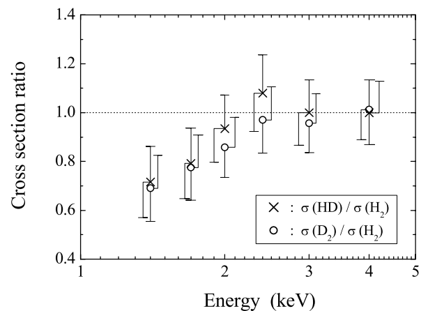
Fig. 6 Charge transfer cross section ratios of HD and \text{D}_2 to \text{H}_2 molecules. Experimental data: ×, HD molecules; ○, \text{D}_2 molecules.
