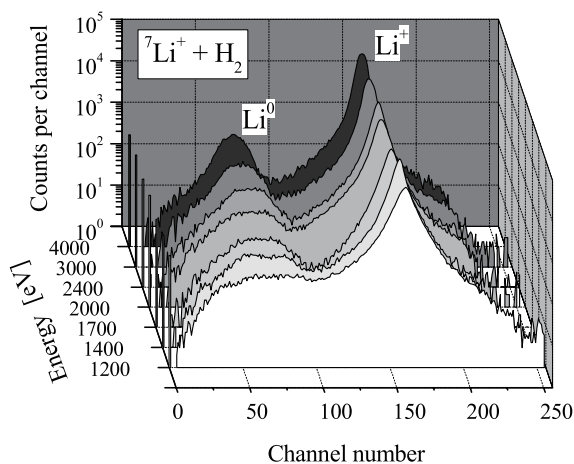
Fig. 4 Charge spectra of incident \text{Li}^+ ions and charge-transferred \text{Li}^0 atoms in \text{Li}^+ + \text{H}_2 collisions. The pressure of target \text{H}_2 gases was about 1 Pa.
