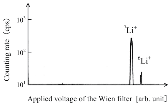
Fig. 2 Typical mass spectrum of lithium extracted from the SIIS. The ion accelerating voltage is 1.7 kV.
