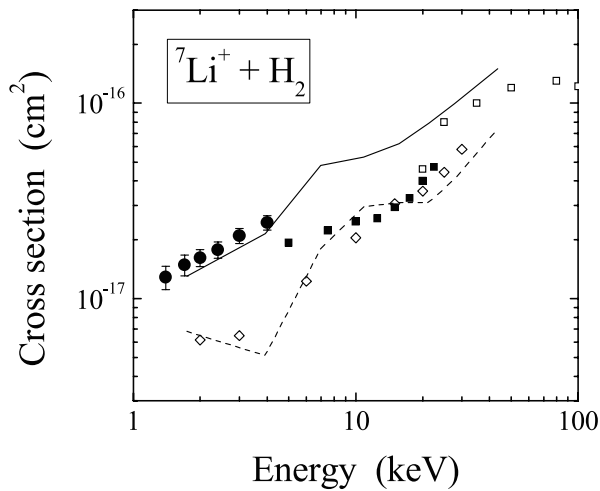
Fig. 3 Charge transfer cross sections of {}^7\text{Li}^+ ions colliding with \text{H}_2 molecules. Experimental data: ●, present data; □, Allison et al. [2]; ■, VanEck and Kistemaker [3]; ◇, Ogurtsov et al. [4]. Theoretical calculation: Elizaga et al. [5] (solid line, transfer to 2l ; broken line, transfer to 2s ).
