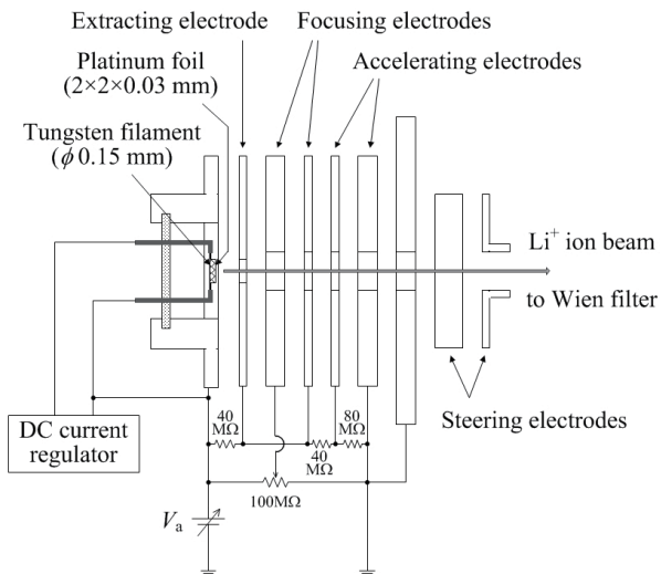
Fig. 1 Cross sectional view of the SIIS and electric circuit for ion extraction.
