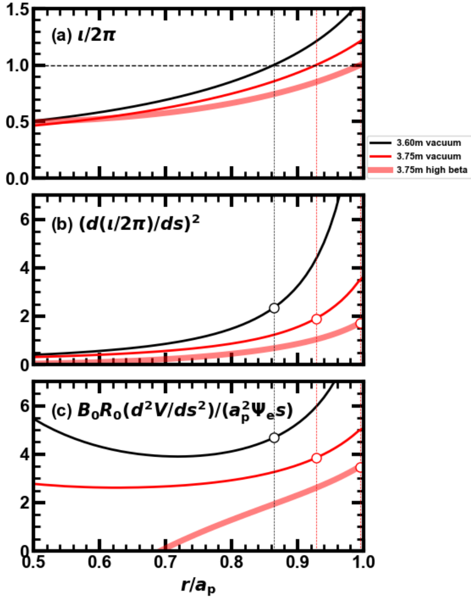
Figure 1. MHD equilibrium characteristics of the LHD. Radial profiles of (a) rotational transform, (b) magnetic shear squared (stabilizing term of Suydam criterion) and (c) magnetic hill index (driving term) with different configurations and conditions. Horizontal axis is the normalized minor radius. Equilibrium parameters are based on a hypothetical VMEC equilibrium under the assumption of beta value and its profile, no plasma current. The black/red lines correspond to a magnetic axis of 3.60/3.75 m in vacuum, and the thick red line to a magnetic axis of 3.75 m at high beta, circles to parameters at l/2\pi = 1 .
