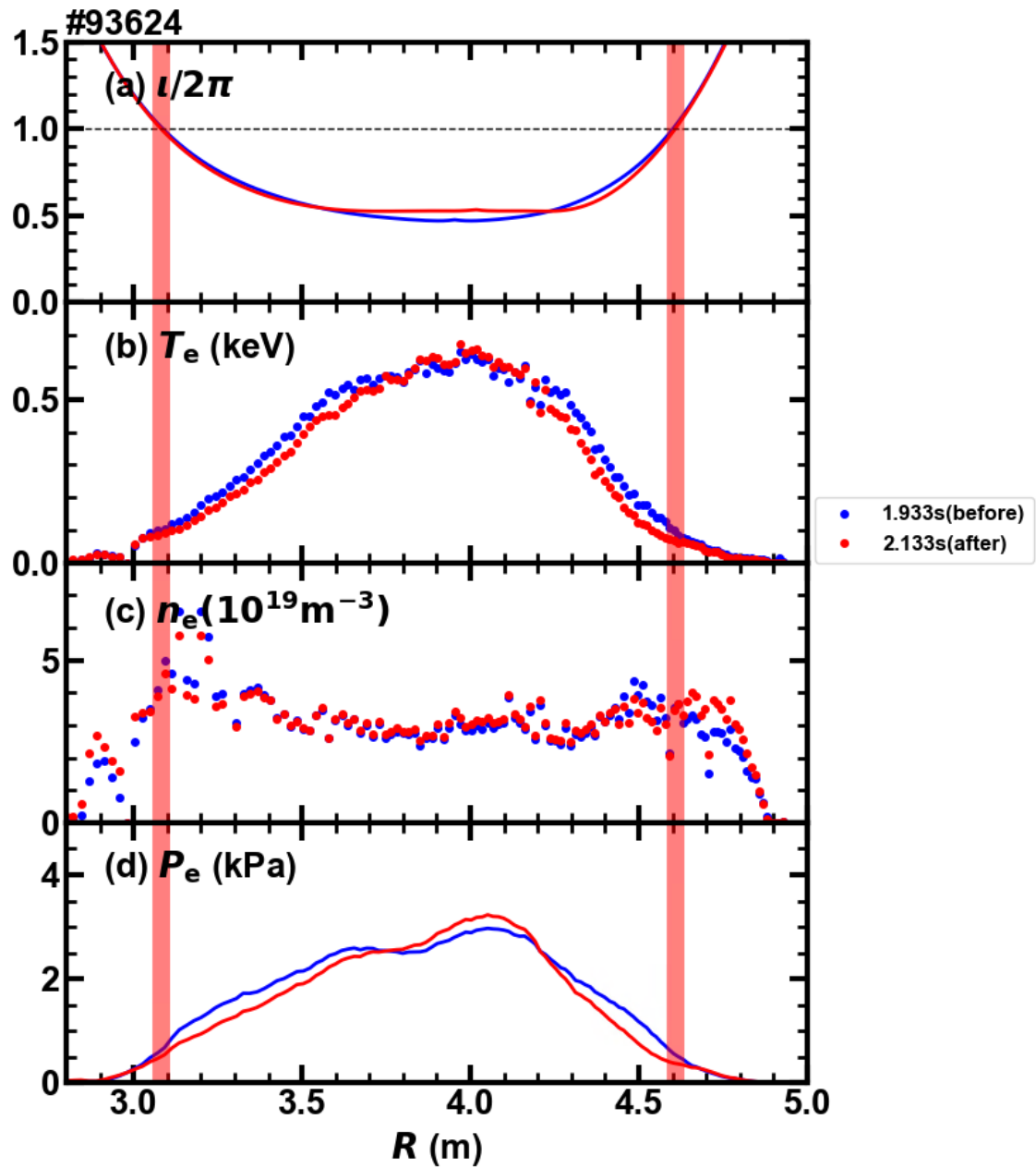
Figure 3. Radial profiles of (a) rotational transform, (b) local electron temperature, (c) local electron density and (d) local electron pressure before (in blue) and at the onset of the instability (in red).
