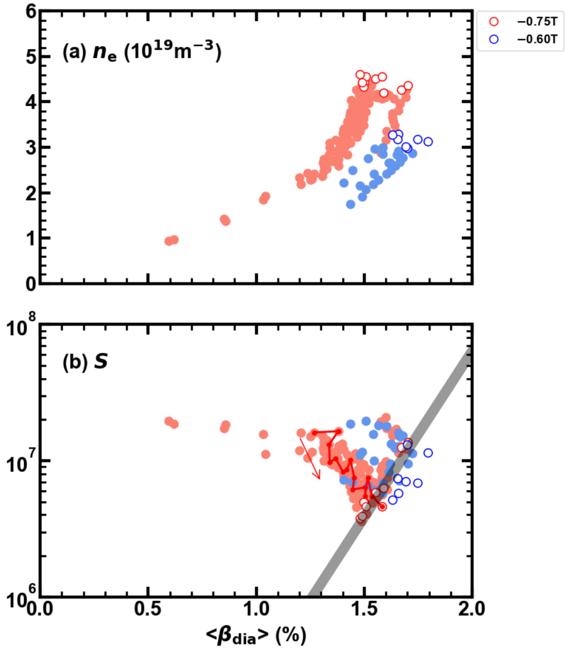
Figure 4. Onset regime of the instability with collapse in the R_{\text{ax}} = 3.75 m configuration in the diagram of beta value and (a) line-averaged electron density and (b) magnetic Reynolds number, S . Filled (open) circles correspond to parameters before (at) the onset of the instability. Red (blue) symbols correspond to parameters at B_t = -0.75 \text{ T} ( -0.60 \text{ T} ) and a red line to time evolution of parameters in the #154036 discharge, as shown in Fig. 5. A black bold line shows the onset conditions of parameters.
