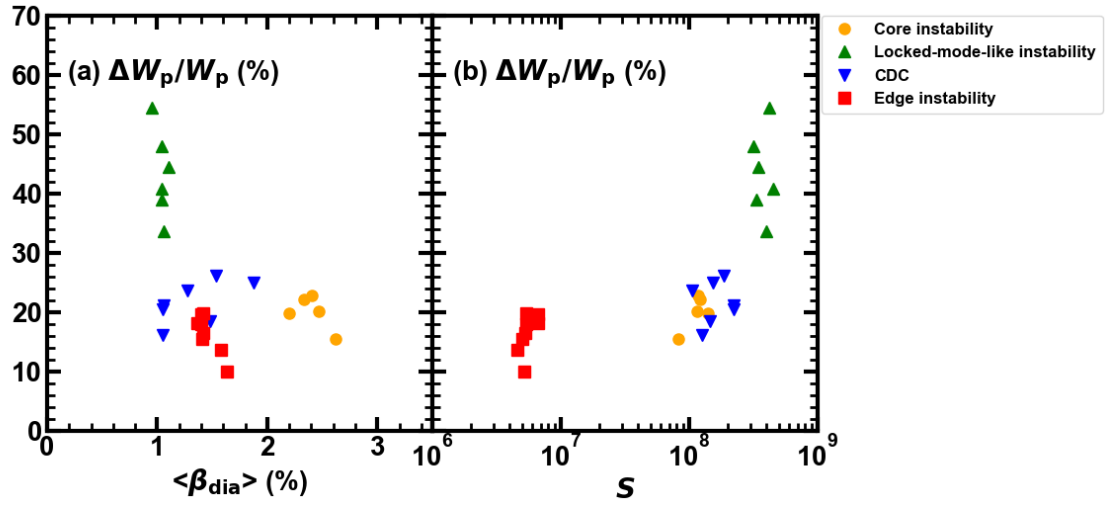
Figure 12. The degradation level of global confinement due to the collapse events and (a) onset volume-averaged beta value and (b) onset magnetic Reynolds number of four types of MHD instabilities observed in the LHD. Red symbols (edge) correspond to instabilities reported in this paper.
