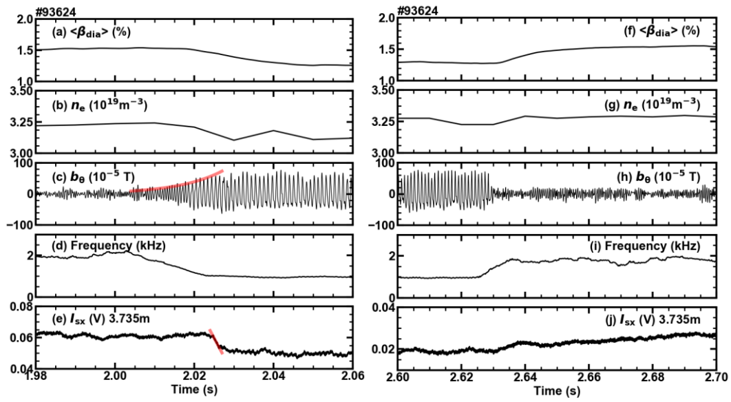
Figure 8. (a)-(e) Appearance process and (f)-(j) disappearance process of the instability. (a)(f) Volume-averaged beta value, (b)(g) line-averaged electron density, (c)(h) a magnetic fluctuation, (d)(i) frequency of the instability and (e)(j) core soft X-ray intensity.
