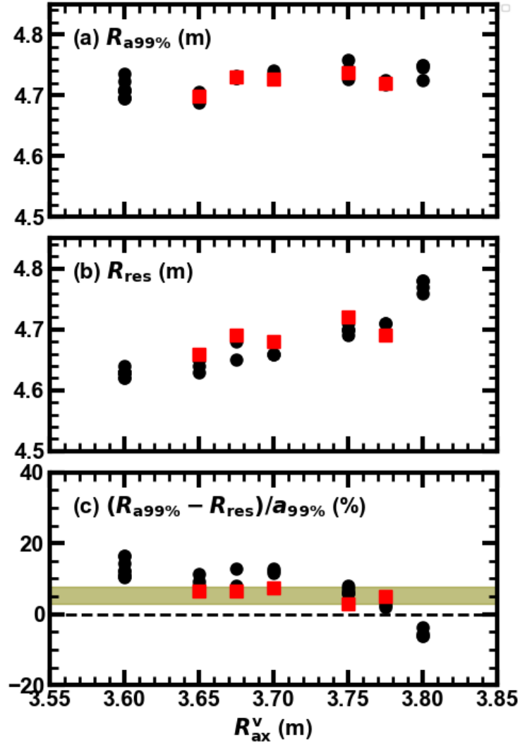
Figure 10. The vacuum magnetic axis location dependence of (a) an index of the plasma boundary, R_{a99\%} , (b) the m/n = 1/1 resonant surface location, R_{res} and (c) the distances between R_{a99\%} and R_{res} . The square symbols correspond to parameters at the instability onset, and the circle symbols to those without the instability. The shaded area displays the region including square symbols for each configuration.
