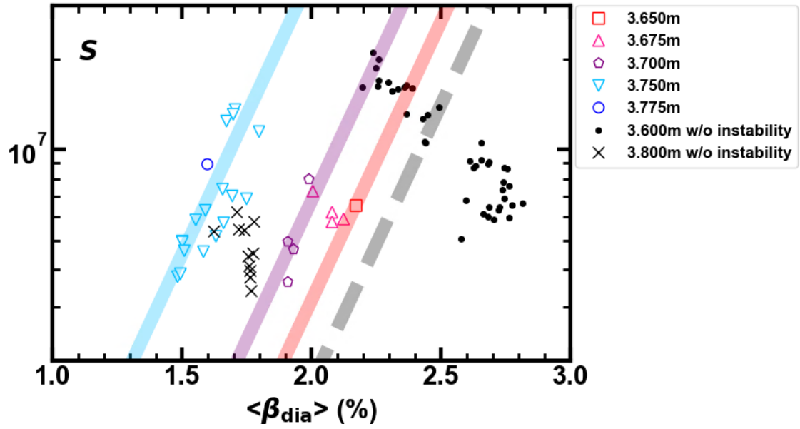
Figure 9. Onset regime with various R_{\text{ax}} configuration in the diagram of beta value and magnetic Reynolds number, S . Parameters with R_{\text{ax}} = 3.75 m are the same as those at the onset, as shown in Fig. 4(b). The auxiliary lines (light blue/purple/red) display the onset conditions of beta and S with various R_{\text{ax}} (3.75/3.70/3.65 m), respectively. Each condition is evaluated from the onset condition with R_{\text{ax}} = 3.75 m and from R_{\text{ax}} dependence of the onset beta. The dashed line corresponds to the estimated onset condition with 3.60 m.
