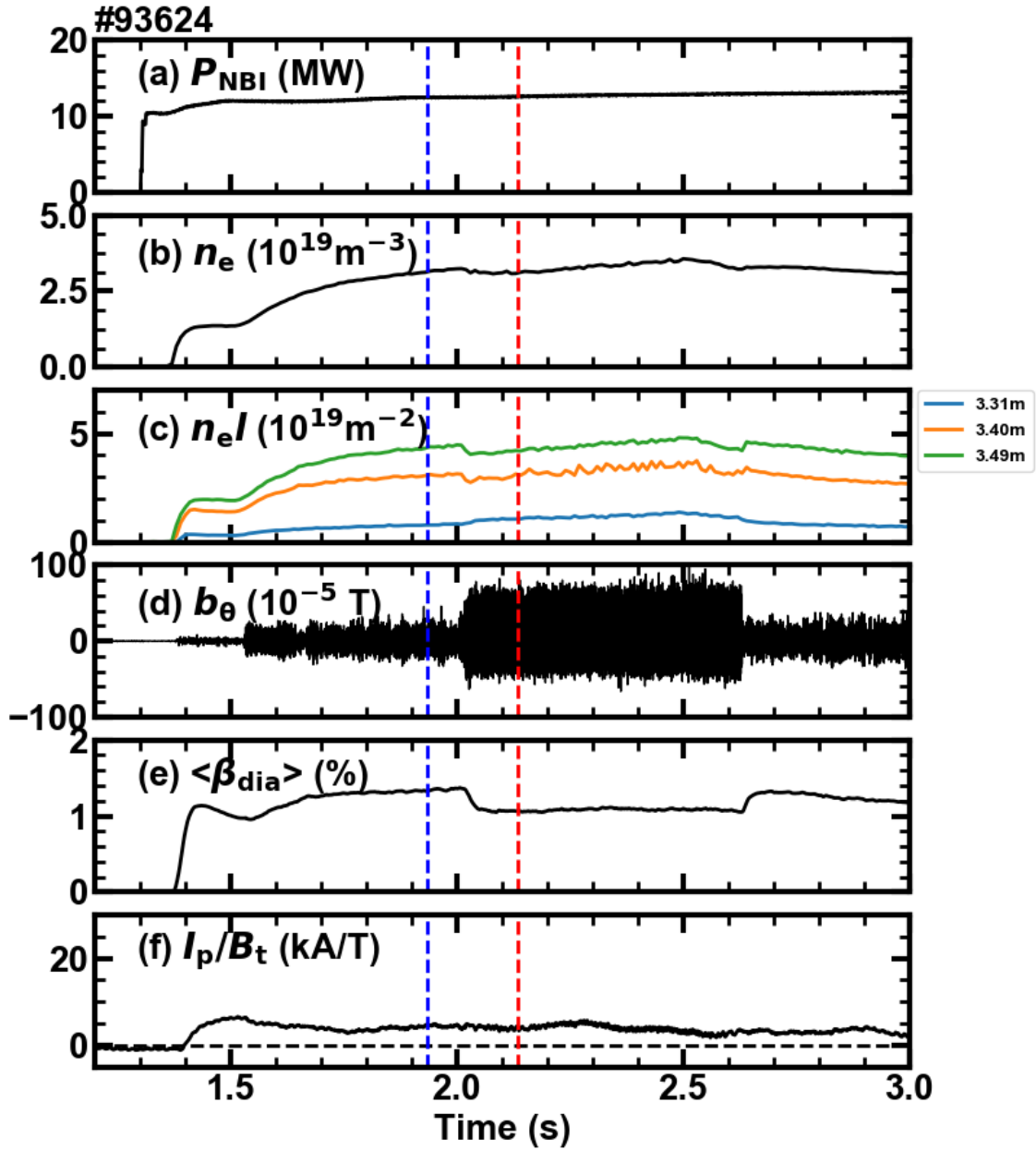
Figure 2. Waveforms of typical discharge where the instability with collapse occurs in the R_{\text{ax}} = 3.75 \text{ m} configuration: (a) total heating power of NBIs, (b) core line-averaged electron density, (c) line-averaged electron density of edge chords of the FIR interferometer, (d) a magnetic fluctuation due to the instability, (e) volume-averaged beta value and (f) plasma current normalized by toroidal magnetic field strength at the magnetic axis.
