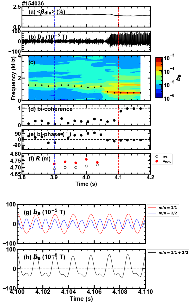
Figure 5. Magnetic fluctuation characteristics of the instability with collapse in the R_{ax} = 3.75 m configuration. (a) Volume-averaged beta value, (b) a magnetic fluctuation, (c) amplitude spectrum of the magnetic fluctuation and frequency of a peak amplitude component in the spectrum ( f_{\text{peak}} , black circles), (d) bi-coherence between three waves with (m, n, \hat{f}) = (1, 1, f_{\text{peak}}) , (1, 1, f_{\text{peak}}) and (2, 2, 2f_{\text{peak}}) , (e) bi-phase and (f) the location of the resonant surface and that of a_{99\%} . Figures 5 (g) and (h) show the m/n = 1/1 and 2/2 magnetic fluctuations and the composite wave during appearance of the instability, respectively. Vertical lines correspond to the timings of the radial mode structure shown in Figs. 7 (d2) and (d3).
