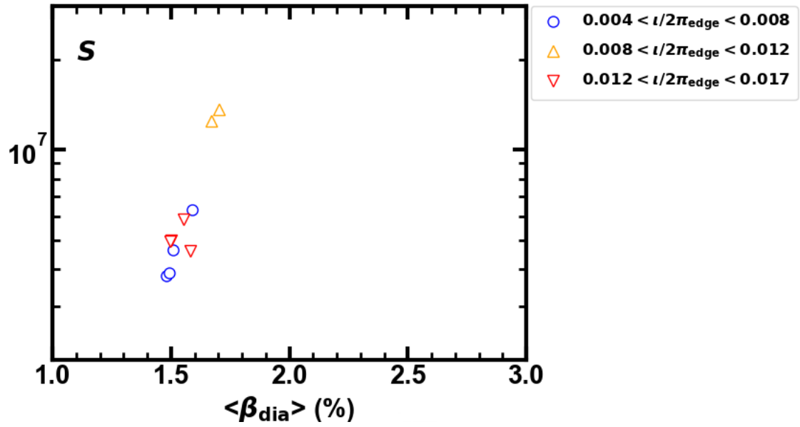
Figure 11. Onset conditions of the instability with collapse in the diagram of beta value and the magnetic Reynolds number, S , for the various plasma current discharges with the R_{\text{ax}} = 3.75 m and B_t = -0.75 T. Here, the current effect is evaluated by the increment of the edge rotational transform due to the current.
