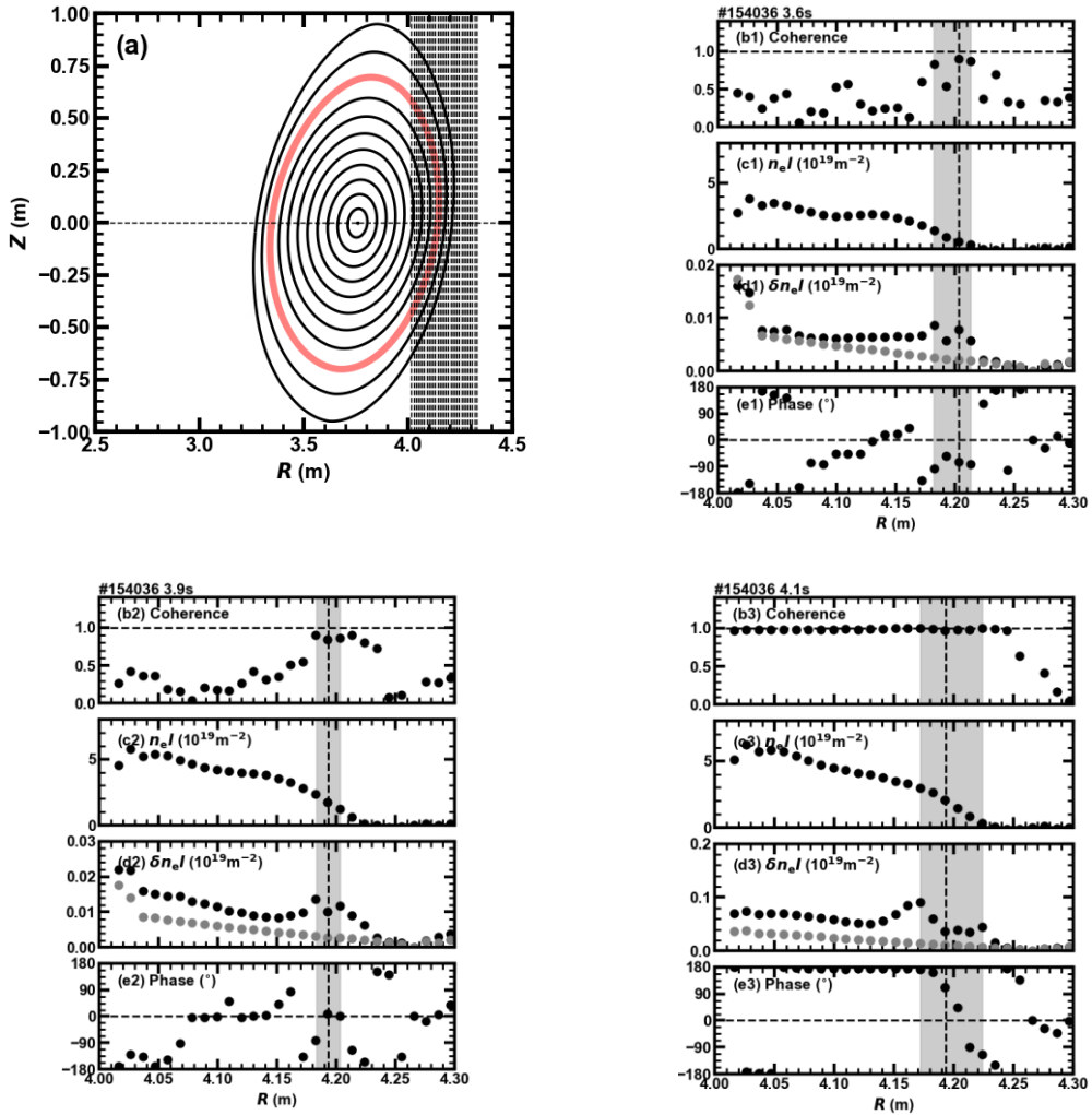
Figure 7. The radial mode structure of m/n = 1/1 fluctuations. (a) Chords of CO 2 laser interferometer. The lines of the magnetic surface are shown every r/a_p = 0.1 and a red thick line corresponds to r/a_p = 1 in the vacuum configuration with R_{ax} = 3.75 m. (b) Coherence between line-averaged electron density fluctuations and a magnetic fluctuation, (c) time-averaged density signals, (d) amplitude of density fluctuations and (e) phase difference between density fluctuations and a magnetic fluctuation before occurrence of the instability at 3.6 s and 3.9 s, and during appearance of the instability at 4.1 s. Grey symbols in the amplitude profiles correspond to the noise level. Hatched area in Figs. 7(b1)-(e1) corresponds to the high coherence region and vertical dashed line displays the peak location within the high coherence region. Hatched areas in Fig. 7(b2)-(e2) and (b3)-(e3) correspond to the region between two peaks and vertical dashed lines display the location of valley between two peaks.
