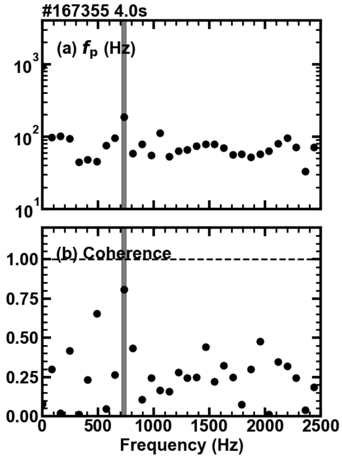
Figure 6. Fourier spectra of the plasma flow velocity signal during appearance of the instability: (a) the flow velocity fluctuation amplitude normalized by the characteristics length and (b) coherence between the flow fluctuation and the magnetic fluctuation. Vertical line corresponds to a high coherent component.
