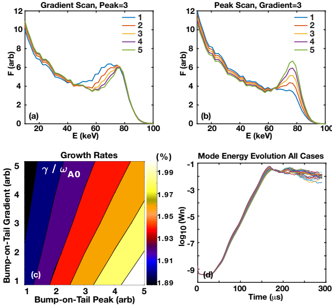
Figure 18. MEGA results for bump-on-tail scan. (a) Range of gradients used at constant peak value. (b) Range of peak values used at constant gradient. (c) Contour of n = 3 TAE growth rates for bump-on-tail scan. (d) Mode energy evolution for all cases.
