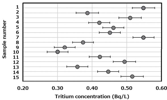
Fig. 3 Tritium concentration in natural spring water at Hirosaki, Japan.
