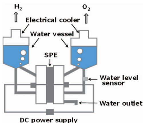
Fig. 2 Overview of SPE electrolytic system.
