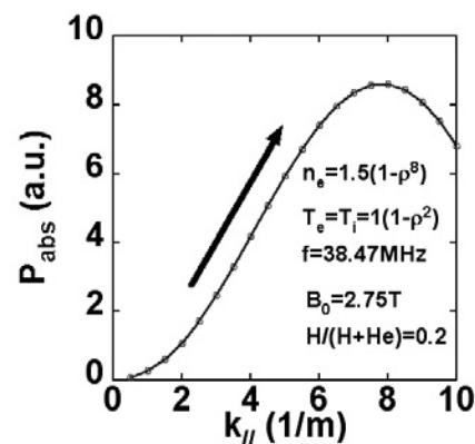
Fig. 2 Power absorption depending on k_{||} .
