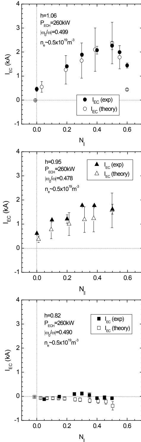
Fig. 1. N_{\parallel} dependence of EC current in three configurations ( h=1.06 , 0.95 and 0.82 ). The closed and open symbols denote the experimental and theoretical EC driven current, respectively.
