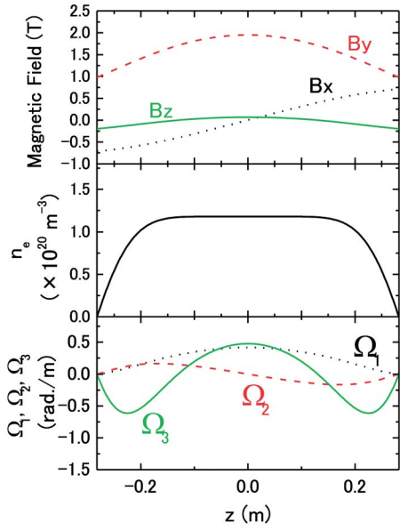
FIG. 1. (Color online) Distributions of the magnetic field components, a typical electron density profile, and components of \Omega along a plasma center chord in a CHS plasma ( R_{\text{ax}}=92.1 cm and B_{\text{ax}}=1.96 T). \Omega is the calculation results in the case of the wavelength of the HCN laser.
