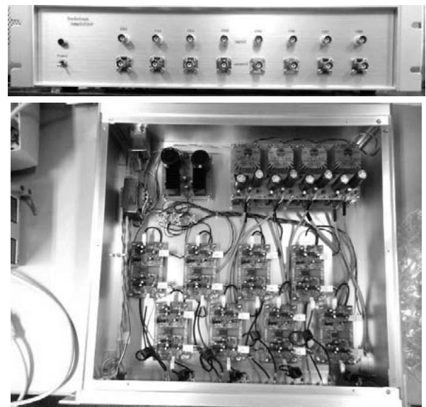
Fig. 2 Front and inside photos of the new 8-channel isolation amplifier: Primary-side power supply is independently implemented for each channel, whereas the secondary-side one is shared with a common (chassis) ground.
