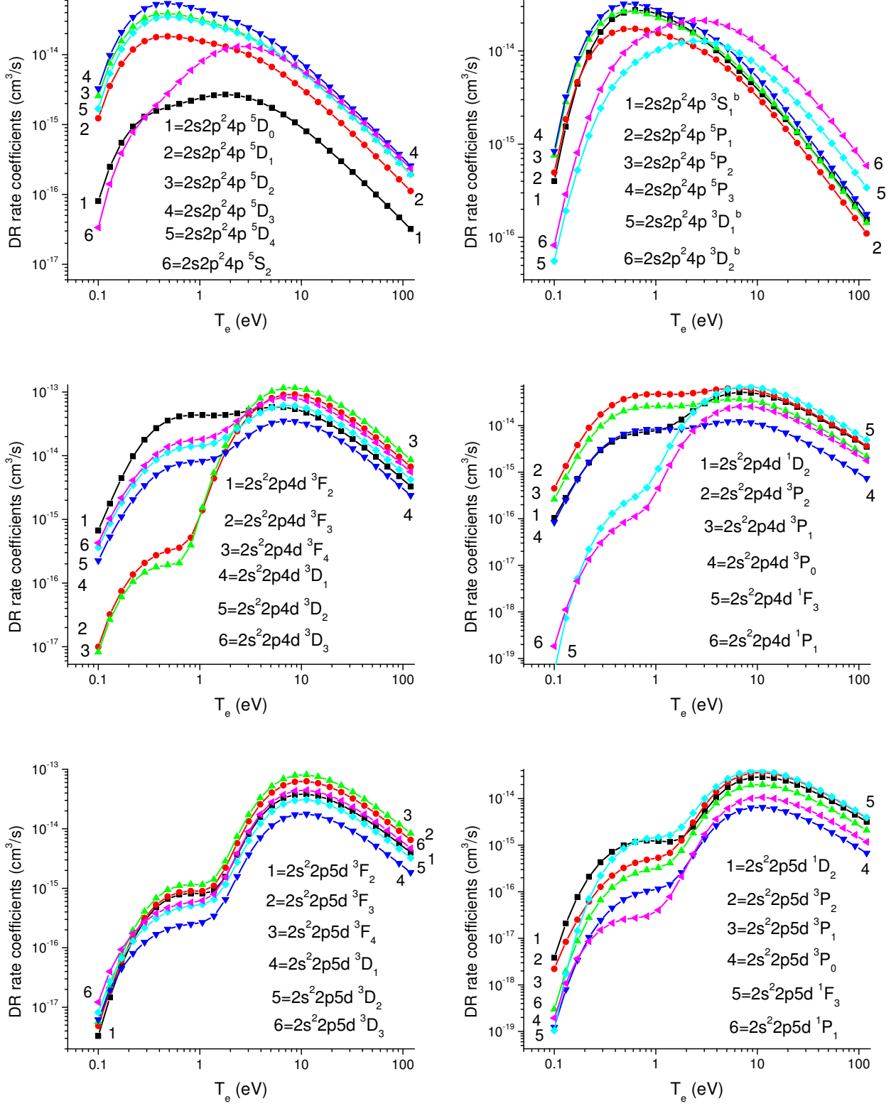
FIG. 16: DR rate coefficients g_0\alpha_d(\gamma|2s^2 2p) for 2s^2 2p^2 4p ^{1,3,5}L_J , 2s^2 2p 4d ^{1,3}L_J , and 2s^2 2p 5d ^{1,3}L_J states as function of T_e in C-like oxygen
