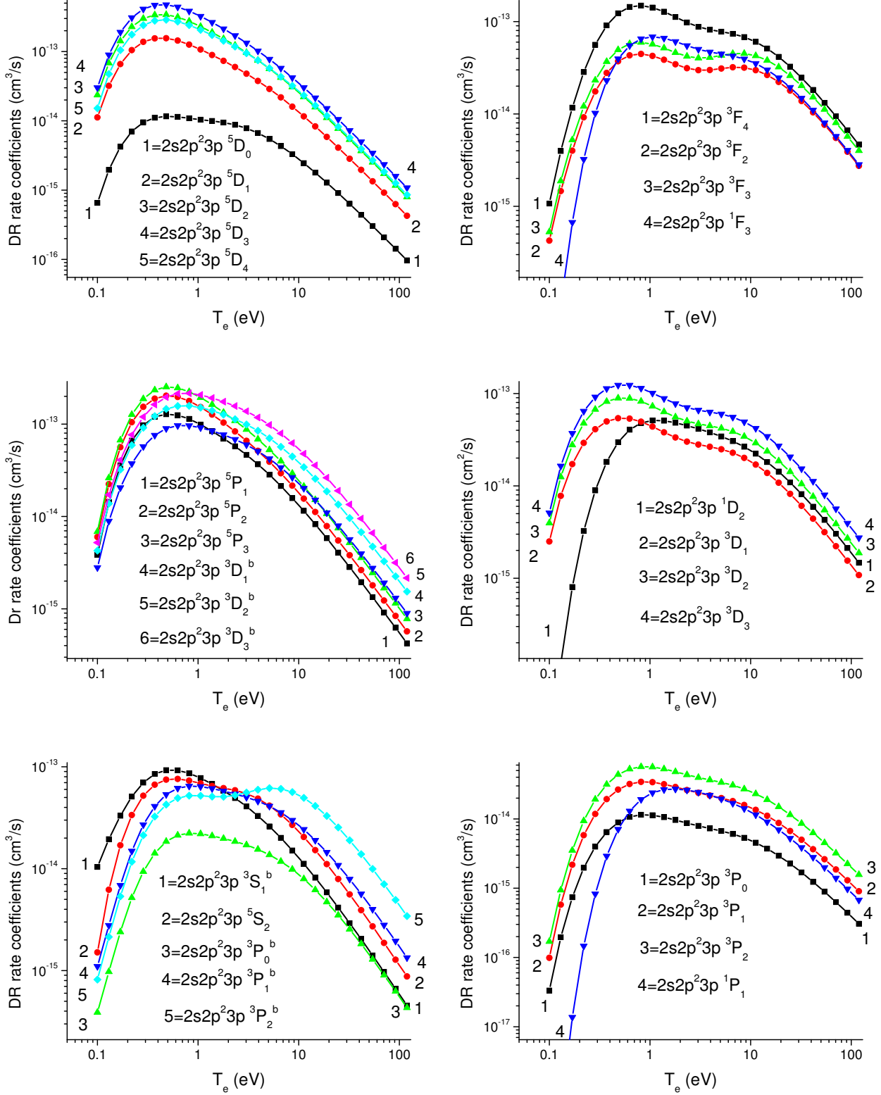
FIG. 15: DR rate coefficients g_0\alpha_d(\gamma|2s^22p) for 2s2p^23p ^{1,3,5}L_J states as function of T_e in C-like oxygen
