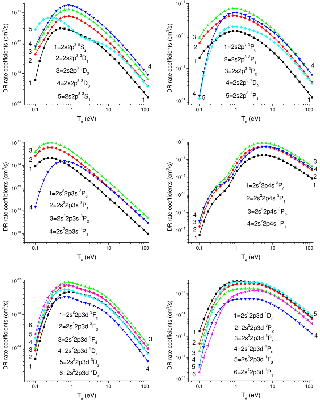
FIG. 14: DR rate coefficients g_0\alpha_d(\gamma|2s^22p) for 2s2p^3\ ^{1,3,5}L_J , 2s^22p3s\ ^{1,3}P_J , 2s^22p4s\ ^{1,3}P_J , and 2s^22p3d\ ^{1,3}L_J states as function of T_e in C-like oxygen
