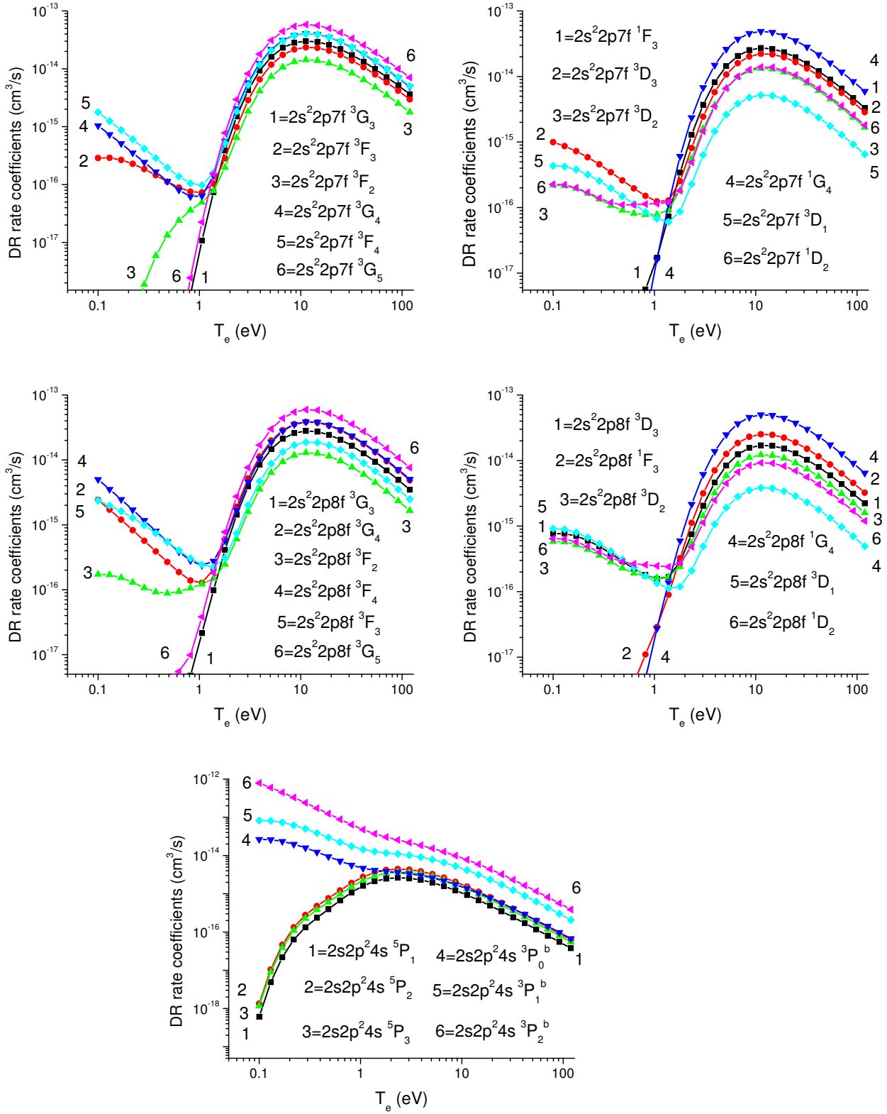
FIG. 13: DR rate coefficients g_0\alpha_d(\gamma|2s^22p) for 2s^22p7f ^{1,3}L_J , 2s^22p8f ^{1,3}L_J , and 2s2p^24s ^{3,5}P_J states as function of T_e in C-like oxygen
