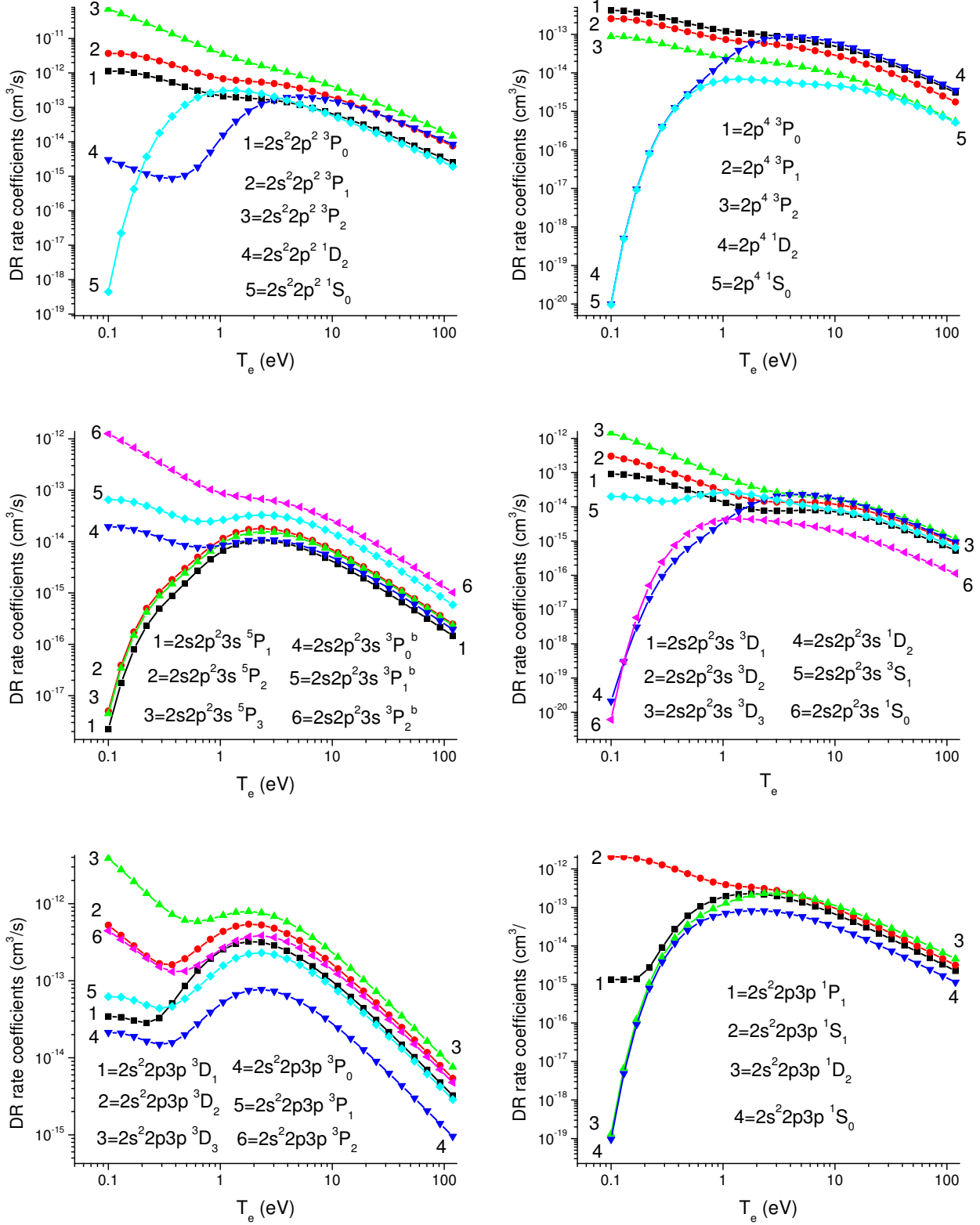
FIG. 8: DR rate coefficients g_0\alpha_d(\gamma|2s^22p) for 2s^22p^2\ ^{1,3}L_J , 2p^4\ ^{1,3}L_J , and 2s^22p3p\ ^{1,3}L_J states as function of T_e in C-like oxygen
