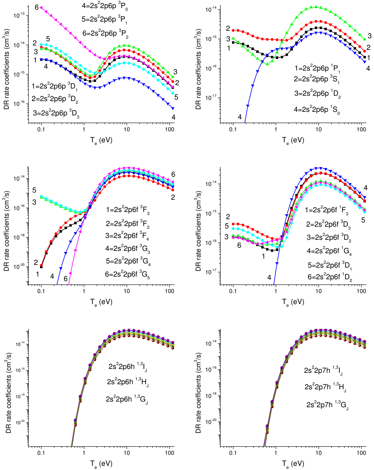
FIG. 11: DR rate coefficients g_0\alpha_d(\gamma|2s^2 2p) for 2s^2 2p6p \ ^{1,3}L_J , 2s^2 2p6f \ ^{1,3}L_J , 2s^2 2p6h \ ^{1,3}L_J , and 2s^2 2p7h \ ^{1,3}L_J states as function of T_e in C-like oxygen
