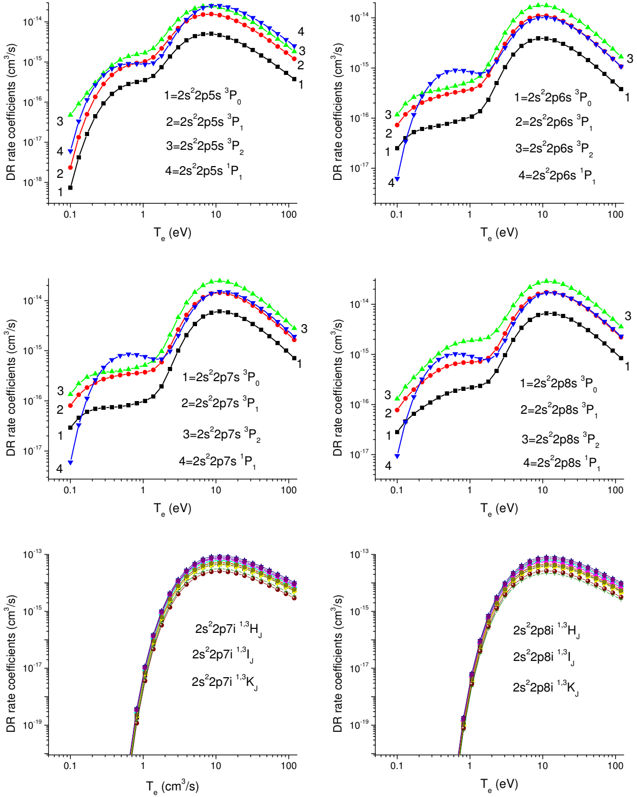
FIG. 17: DR rate coefficients g_0\alpha_d(\gamma|2s^22p) for 2s^22p5s 1,3 P J , 2s^22p6s 1,3 P J , 2s^22p7s 1,3 P J , 2s^22p8s 1,3 P J , 2s^22p7i 1,3 L J , and 2s^22p8i 1,3 L J states as function of T_e in C-like oxygen
