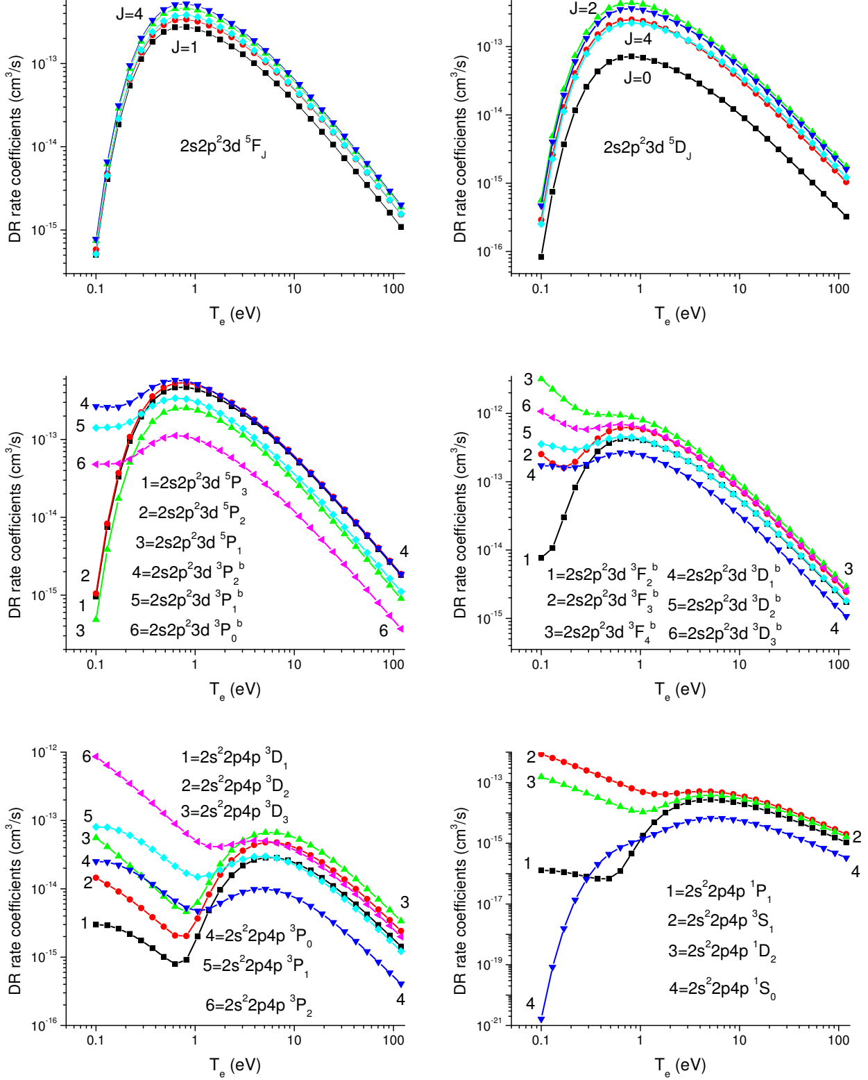
FIG. 9: DR rate coefficients g_0\alpha_d(\gamma|2s^22p) for 2s2p^23d \ ^{1,3,5}L_J and 2s^22p4p \ ^{1,3}L_J states as function of T_e in C-like oxygen
