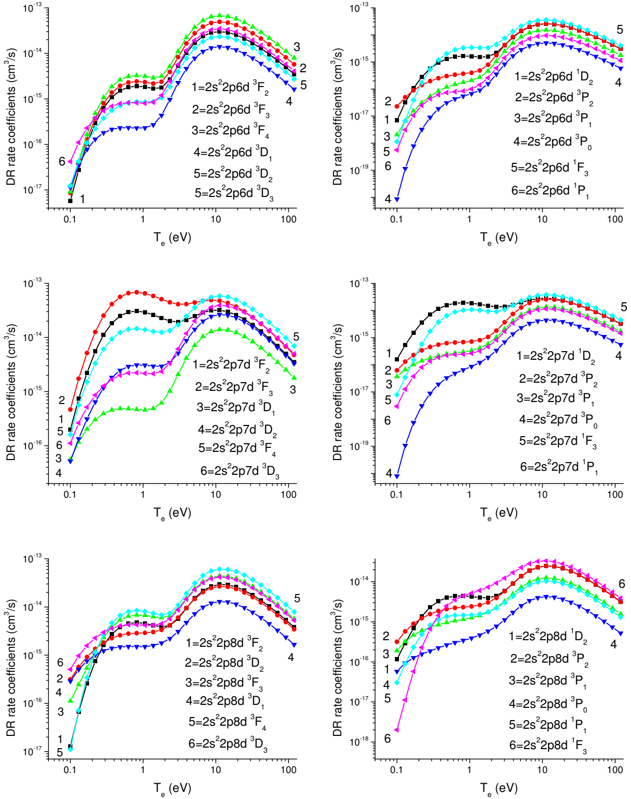
FIG. 18: DR rate coefficients g_0\alpha_d(\gamma|2s^2 2p) for 2s^2 2p 6d \ ^{1,3}L_J , 2s^2 2p 7d \ ^{1,3}L_J , and 2s^2 2p 8d \ ^{1,3}L_J states as function of T_e in C-like oxygen
