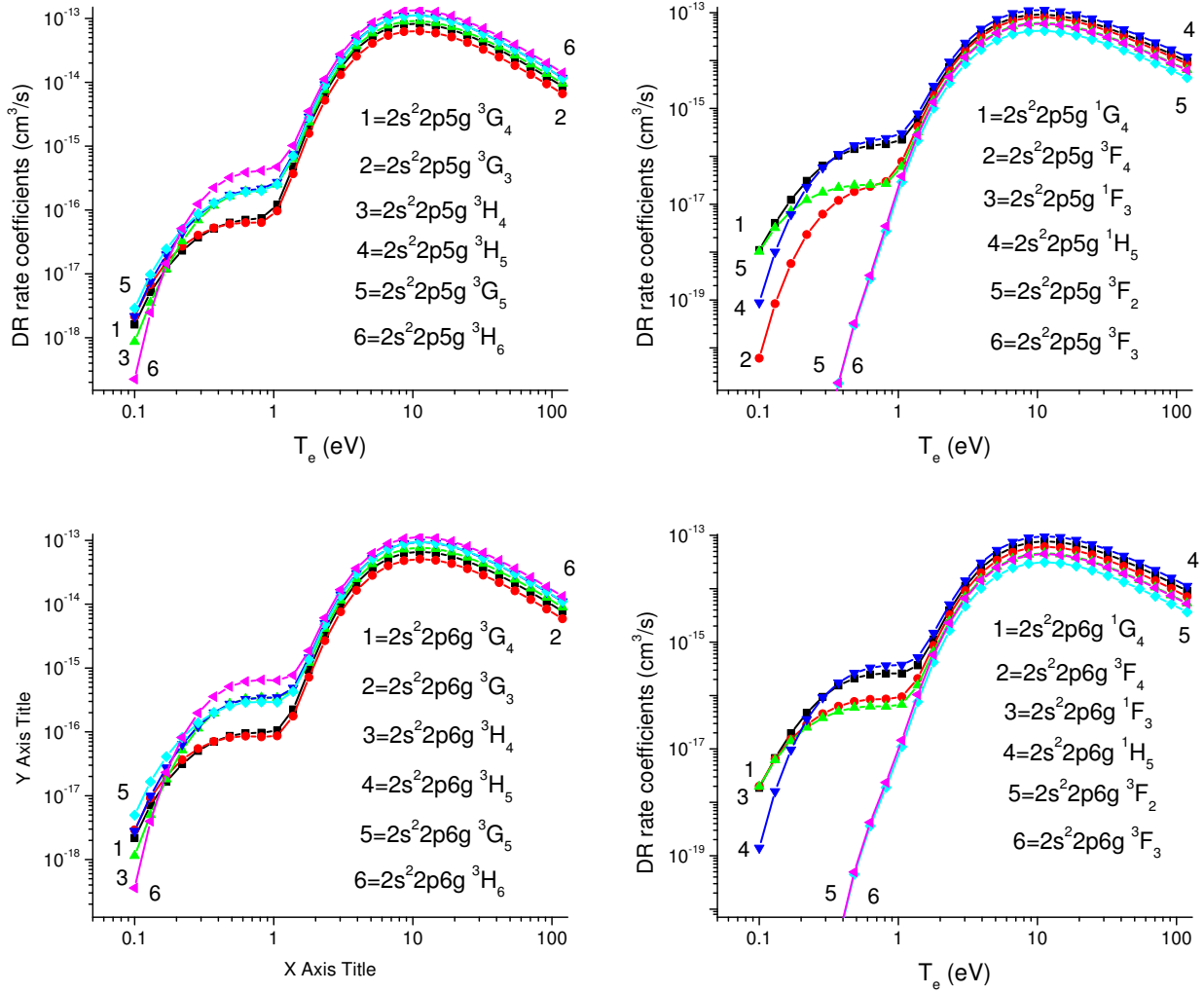
FIG. 19: DR rate coefficients g_0\alpha_d(\gamma|2s^2 2p) for 2s^2 2p5g \ ^{1,3}L_J and 2s^2 2p6g \ ^{1,3}L_J states as function of T_e in C-like oxygen
