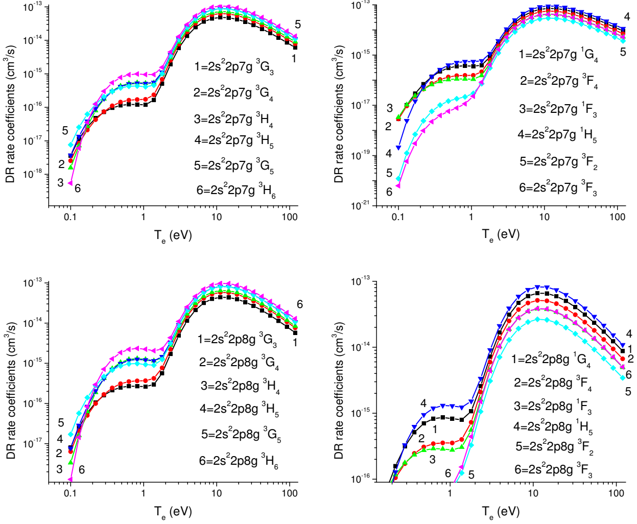
FIG. 20: DR rate coefficients g_0\alpha_d(\gamma|2s^2 2p) for 2s^2 2p 7g \ ^{1,3}L_J and 2s^2 2p 8g \ ^{1,3}L_J states as function of T_e in C-like oxygen
