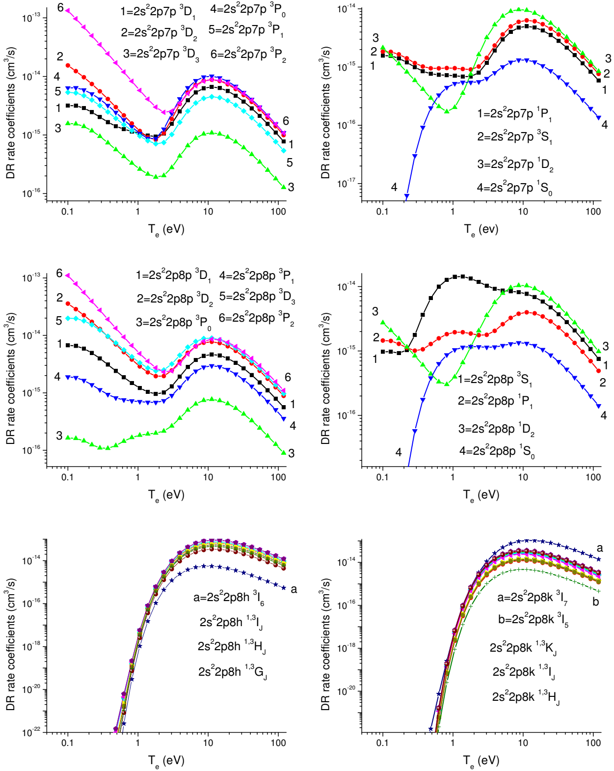
FIG. 12: DR rate coefficient g_0\alpha_d(\gamma|2s^22p) for 2s^22p7p ^{1,3}L_J , 2s^22p8p ^{1,3}L_J , 2s^22p8h ^{1,3}L_J , and 2s^22p8k ^{1,3}L_J states as function of T_e in C-like oxygen
