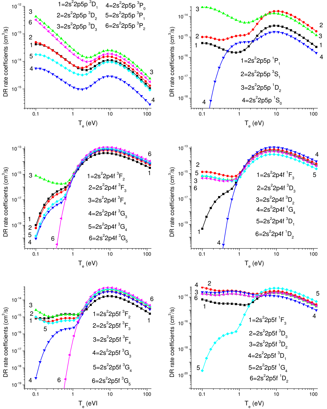
FIG. 10: DR rate coefficients g_0 \alpha_d(\gamma | 2s^2 2p) for 2s^2 2p 5p ^{1,3}L_J , 2s^2 2p 4f ^{1,3}L_J , and 2s^2 2p 5f ^{1,3}L_J states as function of T_e in C-like oxygen
